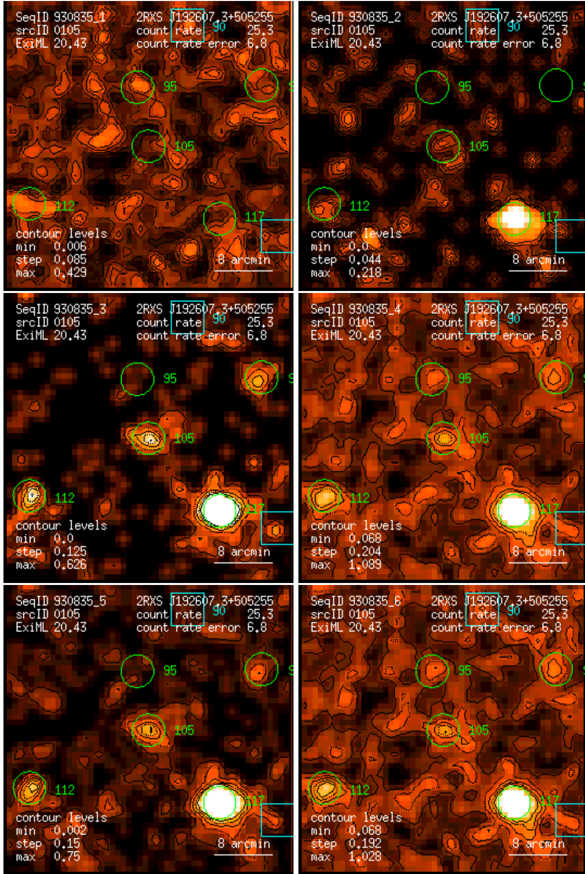
Figure 105: RASS 930835: detection 0105: band rate images, Gaussian filter: (1) PSPC channels 11 – 41, (2) 52 – 90, (3) 91 – 201, (4) 11 – 235, (5) 52 – 201, (6) 11 – 201. Broad band rates in counts/ks. Band rate contour levels in counts/ks/arcmin 2 .
