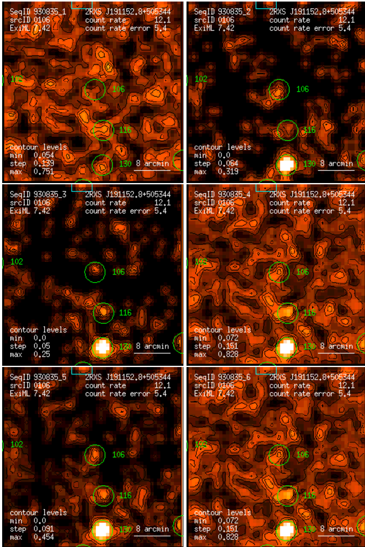
Figure 106: RASS 930835: detection 0106: band rate images, Gaussian filter: (1) PSPC channels 11 – 41, (2) 52 – 90, (3) 91 – 201, (4) 11 – 235, (5) 52 – 201, (6) 11 – 201. Broad band rates in counts/ks. Band rate contour levels in counts/ks/arcmin 2 .
