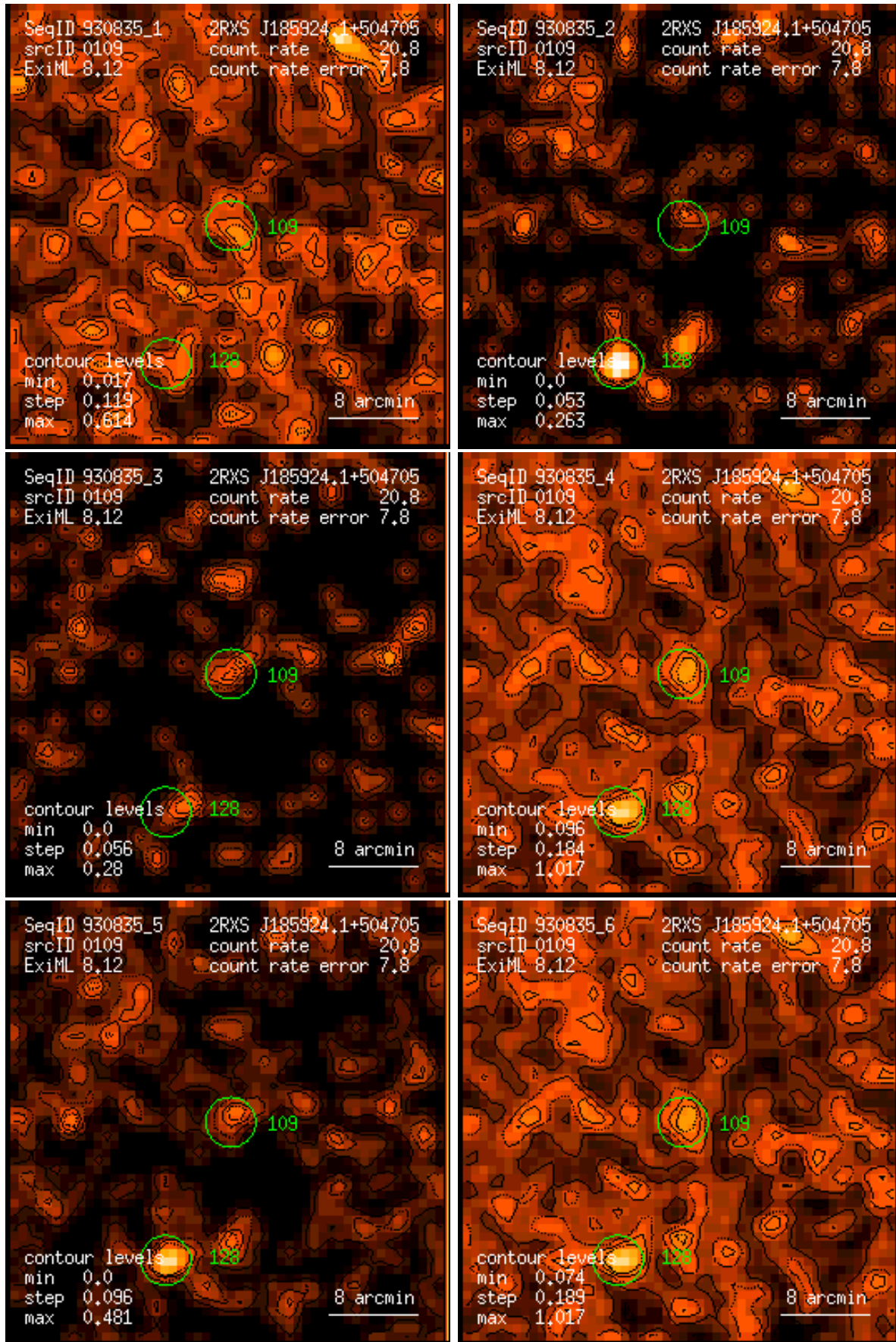
Figure 109: RASS 930835: detection 0109: band rate images, Gaussian filter: (1) PSPC channels 11 – 41, (2) 52 – 90, (3) 91 – 201, (4) 11 – 235, (5) 52 – 201, (6) 11 – 201. Broad band rates in counts/ks. Band rate contour levels in counts/ks/arcmin 2 .
