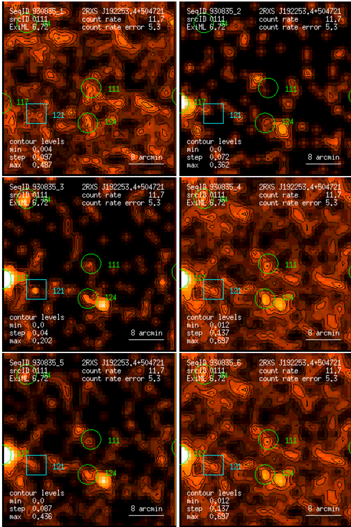
Figure 111: RASS 930835: detection 0111: band rate images, Gaussian filter: (1) PSPC channels 11 – 41, (2) 52 – 90, (3) 91 – 201, (4) 11 – 235, (5) 52 – 201, (6) 11 – 201. Broad band rates in counts/ks. Band rate contour levels in counts/ks/arcmin 2 .
