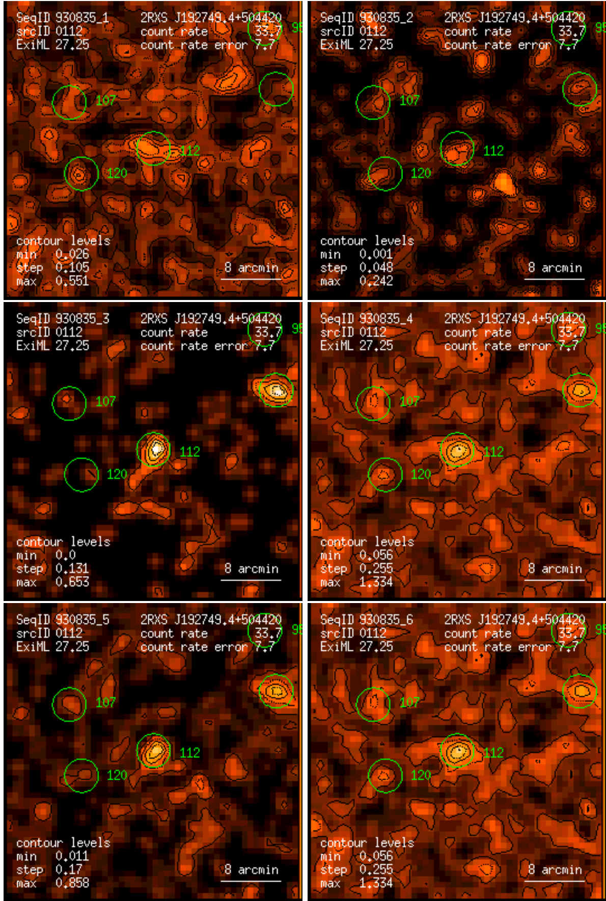
Figure 112: RASS 930835: detection 0112: band rate images, Gaussian filter: (1) PSPC channels 11 – 41, (2) 52 – 90, (3) 91 – 201, (4) 11 – 235, (5) 52 – 201, (6) 11 – 201. Broad band rates in counts/ks. Band rate contour levels in counts/ks/arcmin 2 .
