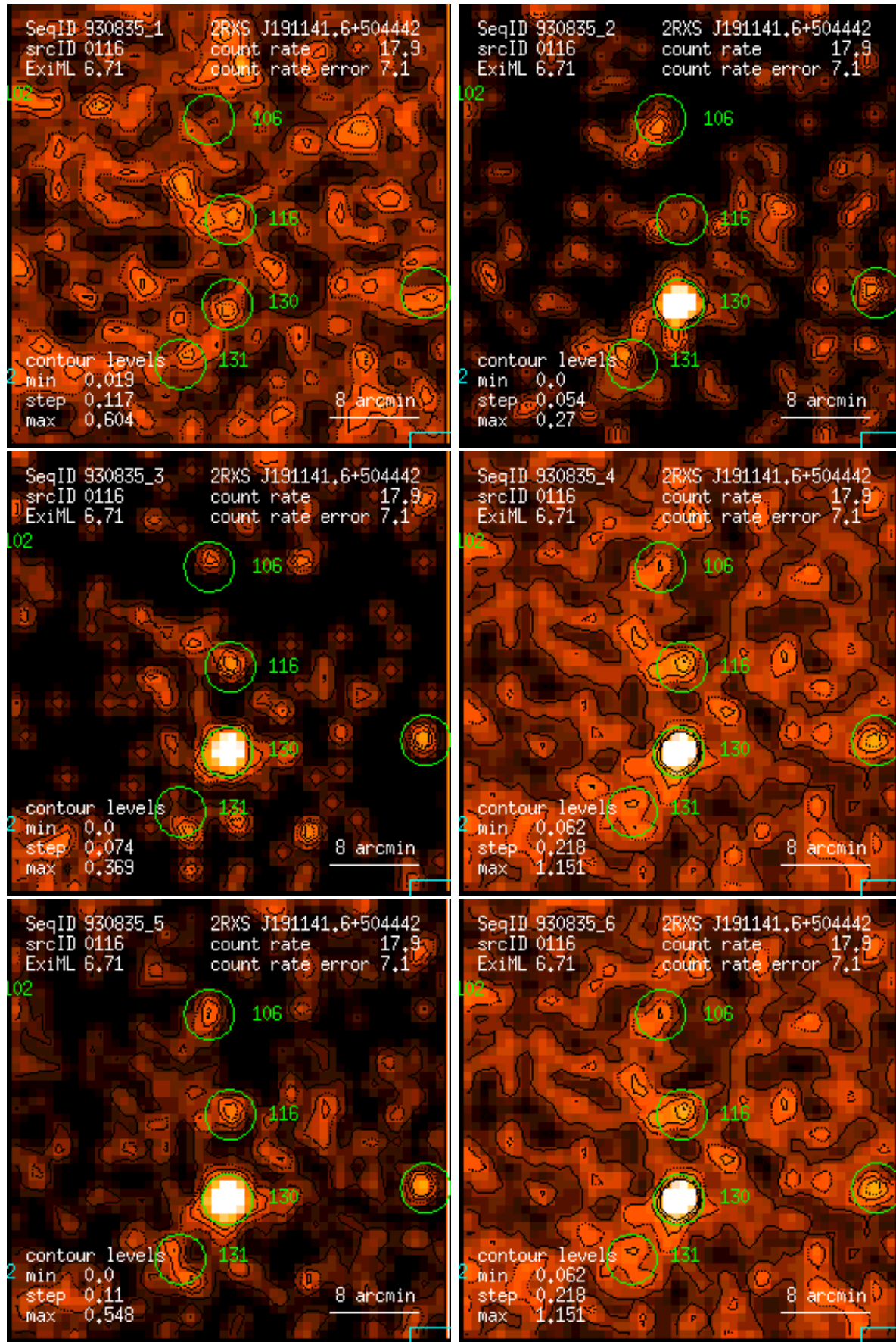
Figure 116: RASS 930835: detection 0116: band rate images, Gaussian filter: (1) PSPC channels 11 – 41, (2) 52 – 90, (3) 91 – 201, (4) 11 – 235, (5) 52 – 201, (6) 11 – 201. Broad band rates in counts/ks. Band rate contour levels in counts/ks/arcmin 2 .
