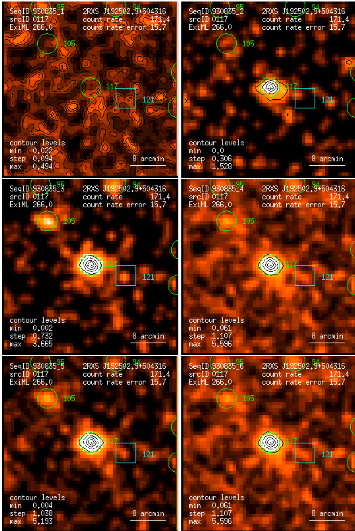
Figure 117: RASS 930835: detection 0117: band rate images, Gaussian filter: (1) PSPC channels 11 – 41, (2) 52 – 90, (3) 91 – 201, (4) 11 – 235, (5) 52 – 201, (6) 11 – 201. Broad band rates in counts/ks. Band rate contour levels in counts/ks/arcmin 2 .
