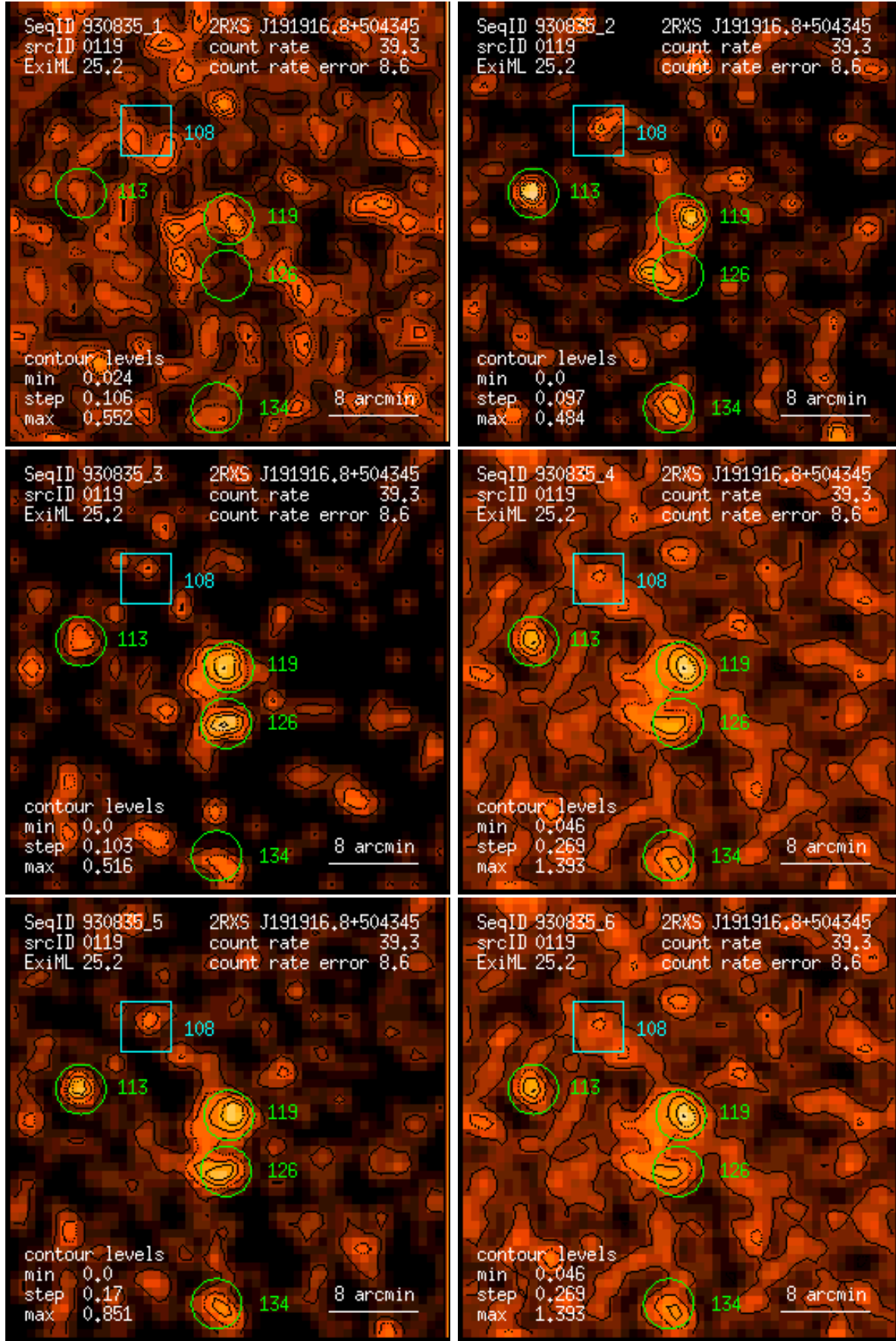
Figure 119: RASS 930835: detection 0119: band rate images, Gaussian filter: (1) PSPC channels 11 – 41, (2) 52 – 90, (3) 91 – 201, (4) 11 – 235, (5) 52 – 201, (6) 11 – 201. Broad band rates in counts/ks. Band rate contour levels in counts/ks/arcmin 2 .
