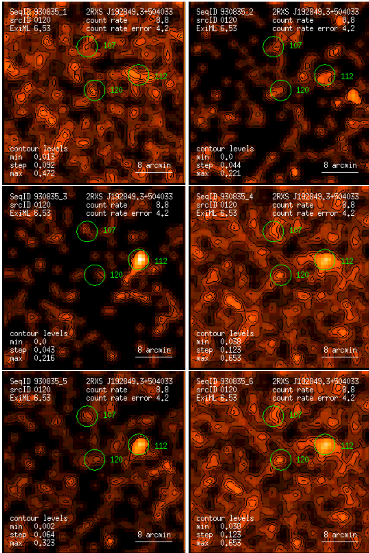
Figure 120: RASS 930835: detection 0120: band rate images, Gaussian filter: (1) PSPC channels 11 – 41, (2) 52 – 90, (3) 91 – 201, (4) 11 – 235, (5) 52 – 201, (6) 11 – 201. Broad band rates in counts/ks. Band rate contour levels in counts/ks/arcmin 2 .
