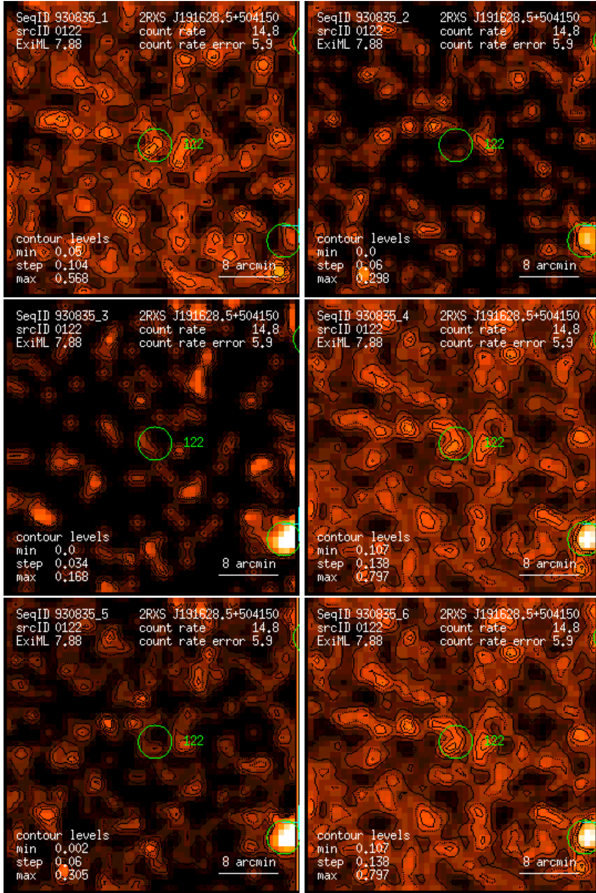
Figure 122: RASS 930835: detection 0122: band rate images, Gaussian filter: (1) PSPC channels 11 – 41, (2) 52 – 90, (3) 91 – 201, (4) 11 – 235, (5) 52 – 201, (6) 11 – 201. Broad band rates in counts/ks. Band rate contour levels in counts/ks/arcmin 2 .
