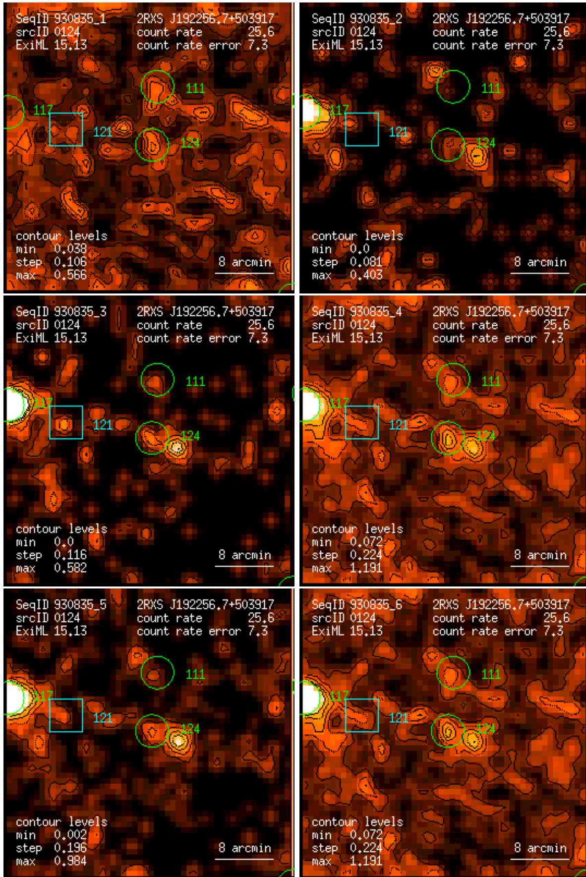
Figure 124: RASS 930835: detection 0124: band rate images, Gaussian filter: (1) PSPC channels 11 – 41, (2) 52 – 90, (3) 91 – 201, (4) 11 – 235, (5) 52 – 201, (6) 11 – 201. Broad band rates in counts/ks. Band rate contour levels in counts/ks/arcmin 2 .
