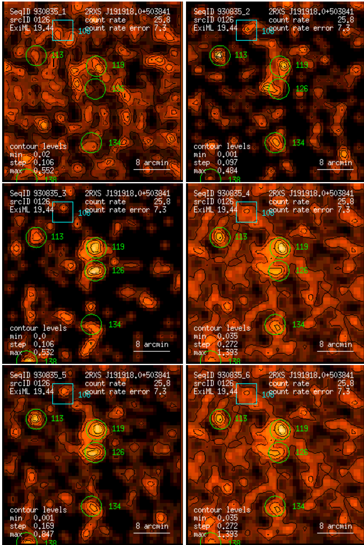
Figure 126: RASS 930835: detection 0126: band rate images, Gaussian filter: (1) PSPC channels 11 – 41, (2) 52 – 90, (3) 91 – 201, (4) 11 – 235, (5) 52 – 201, (6) 11 – 201. Broad band rates in counts/ks. Band rate contour levels in counts/ks/arcmin 2 .
