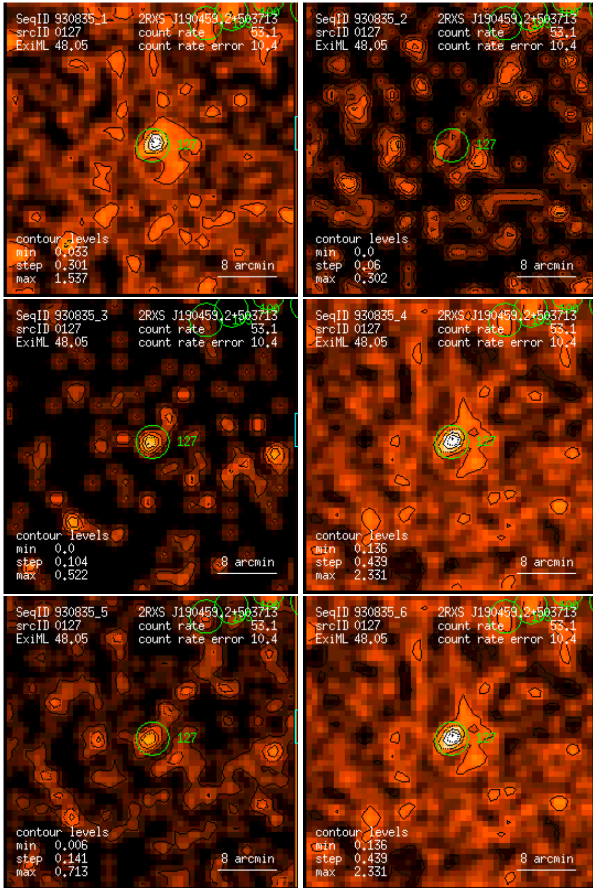
Figure 127: RASS 930835: detection 0127: band rate images, Gaussian filter: (1) PSPC channels 11 – 41, (2) 52 – 90, (3) 91 – 201, (4) 11 – 235, (5) 52 – 201, (6) 11 – 201. Broad band rates in counts/ks. Band rate contour levels in counts/ks/arcmin 2 .
