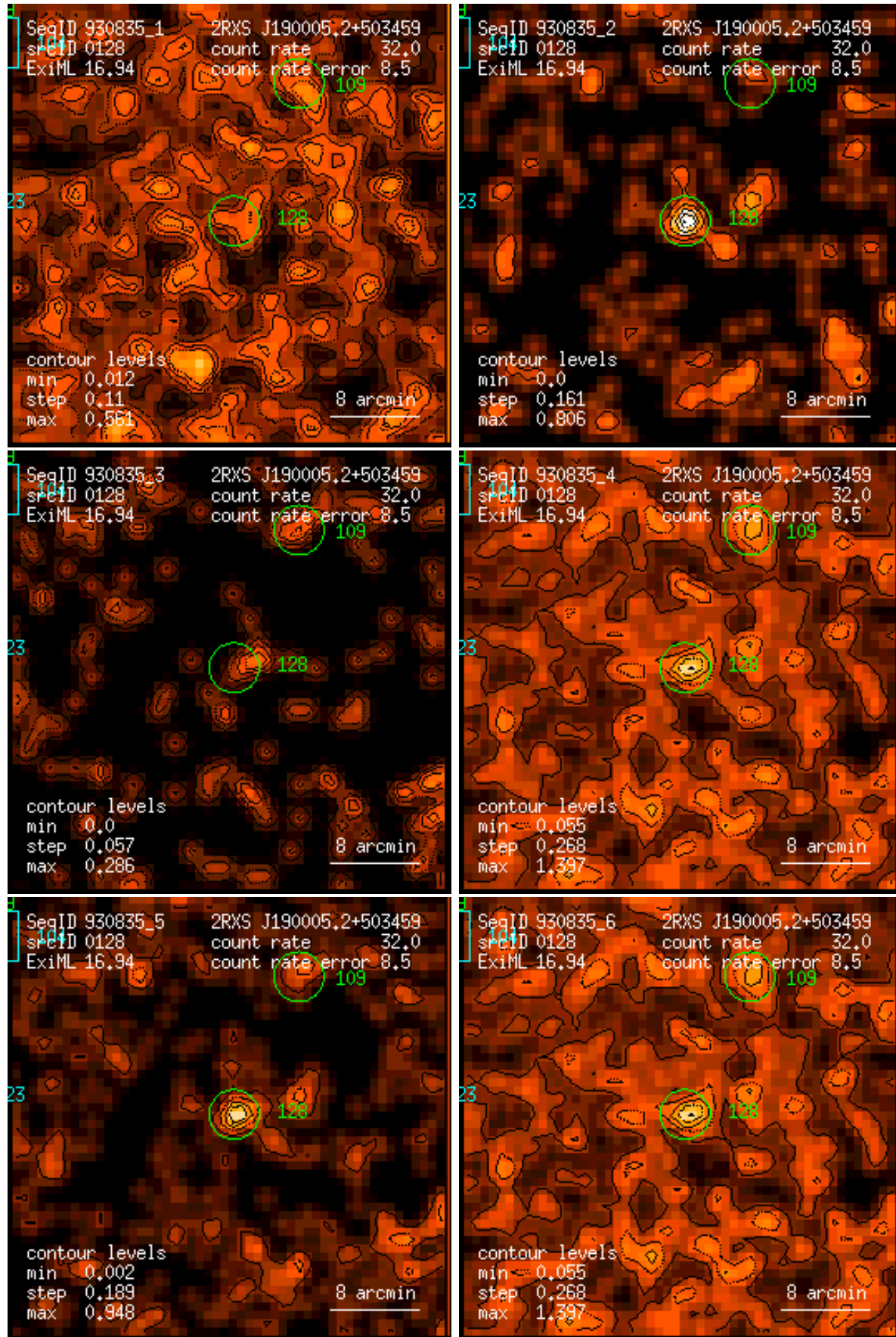
Figure 128: RASS 930835: detection 0128: band rate images, Gaussian filter: (1) PSPC channels 11 – 41, (2) 52 – 90, (3) 91 – 201, (4) 11 – 235, (5) 52 – 201, (6) 11 – 201. Broad band rates in counts/ks. Band rate contour levels in counts/ks/arcmin 2 .
