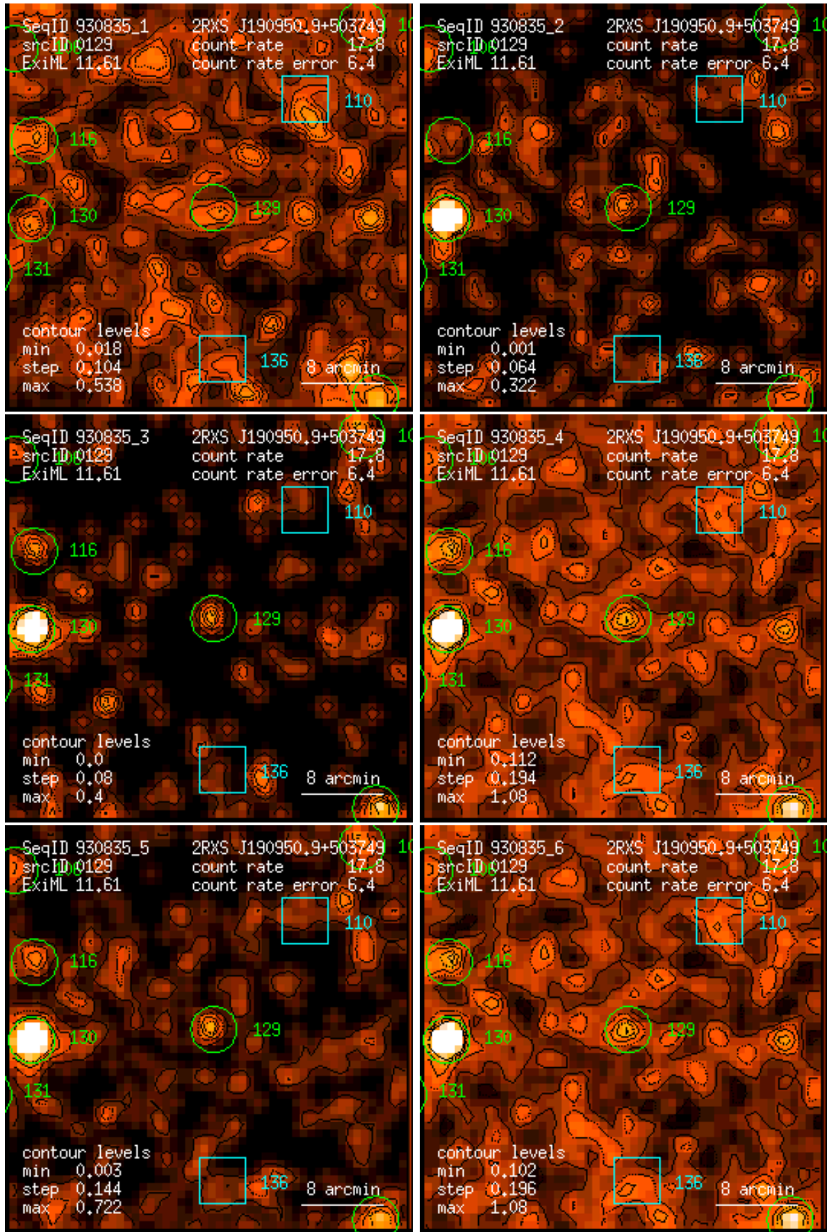
Figure 129: RASS 930835: detection 0129: band rate images, Gaussian filter: (1) PSPC channels 11 – 41, (2) 52 – 90, (3) 91 – 201, (4) 11 – 235, (5) 52 – 201, (6) 11 – 201. Broad band rates in counts/ks. Band rate contour levels in counts/ks/arcmin 2 .
