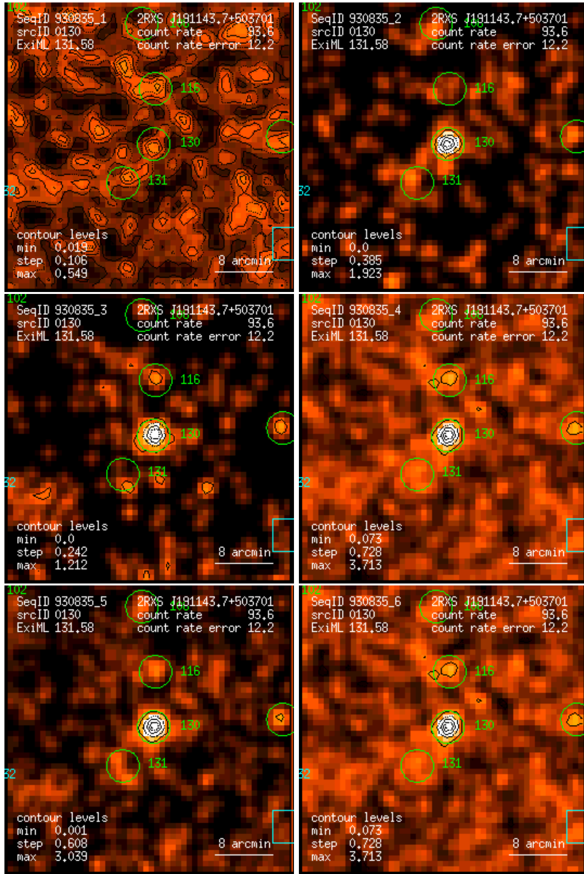
Figure 130: RASS 930835: detection 0130: band rate images, Gaussian filter: (1) PSPC channels 11 – 41, (2) 52 – 90, (3) 91 – 201, (4) 11 – 235, (5) 52 – 201, (6) 11 – 201. Broad band rates in counts/ks. Band rate contour levels in counts/ks/arcmin 2 .
