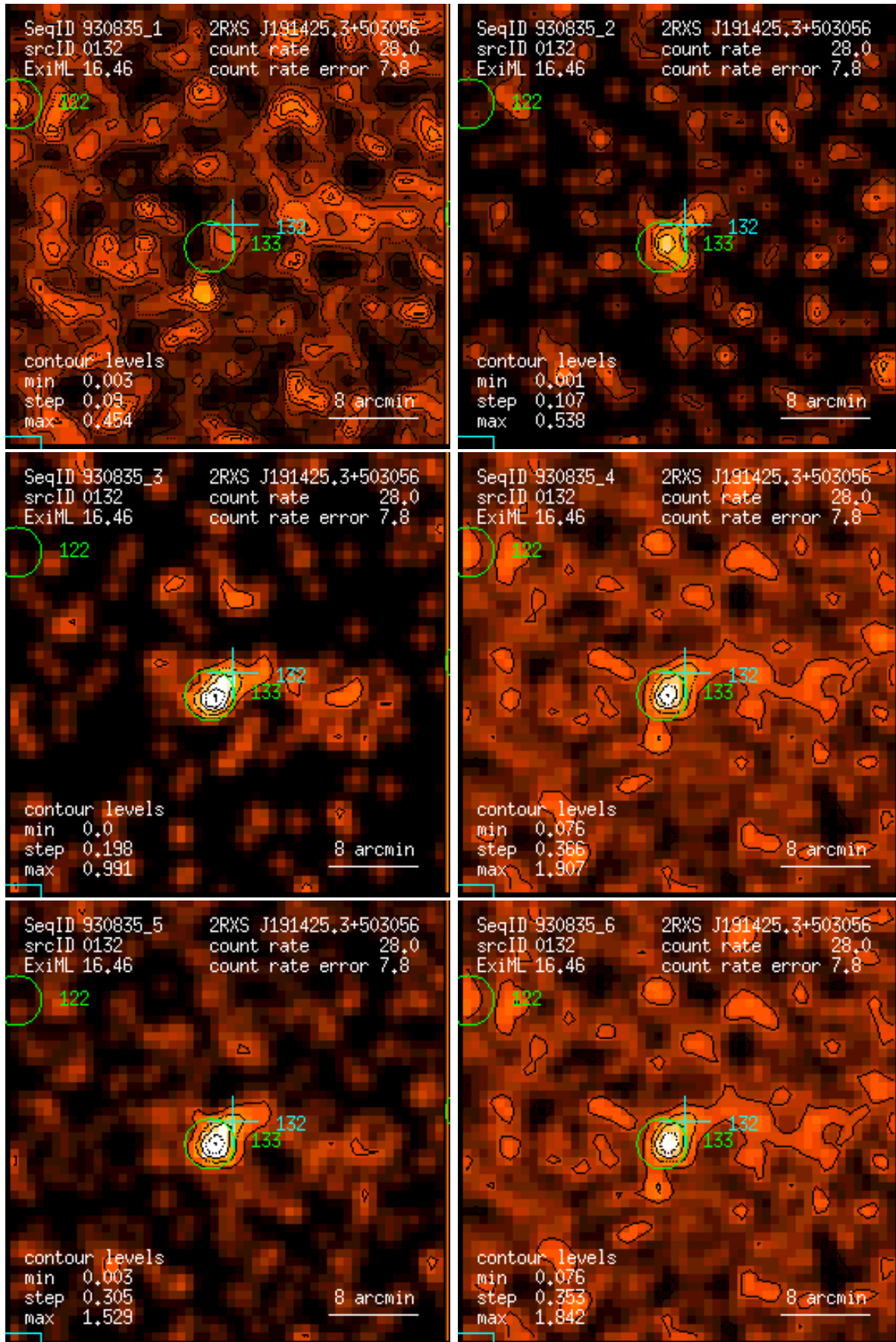
Figure 132: RASS 930835: detection 0132: band rate images, Gaussian filter: (1) PSPC channels 11 – 41, (2) 52 – 90, (3) 91 – 201, (4) 11 – 235, (5) 52 – 201, (6) 11 – 201. Broad band rates in counts/ks. Band rate contour levels in counts/ks/arcmin 2 .
