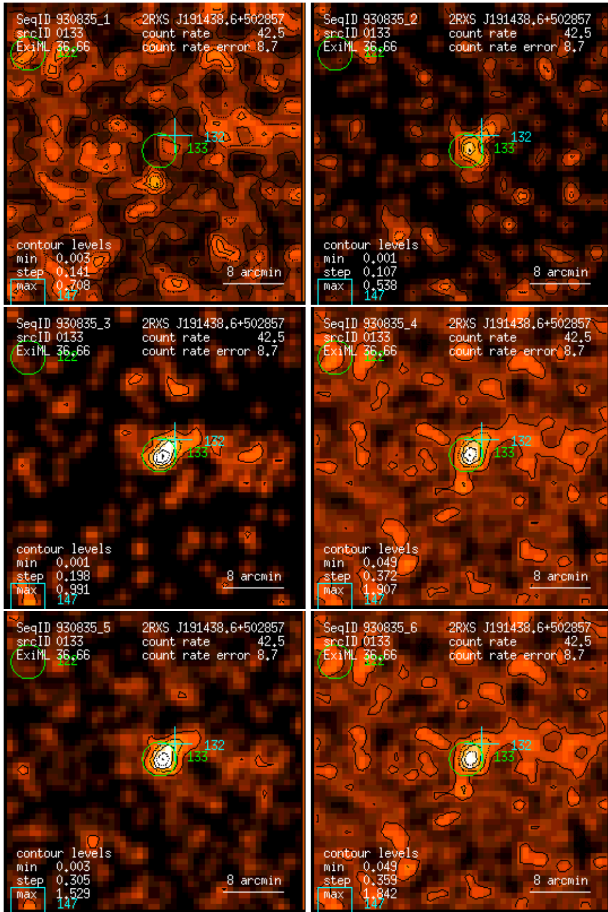
Figure 133: RASS 930835: detection 0133: band rate images, Gaussian filter: (1) PSPC channels 11 – 41, (2) 52 – 90, (3) 91 – 201, (4) 11 – 235, (5) 52 – 201, (6) 11 – 201. Broad band rates in counts/ks. Band rate contour levels in counts/ks/arcmin 2 .
