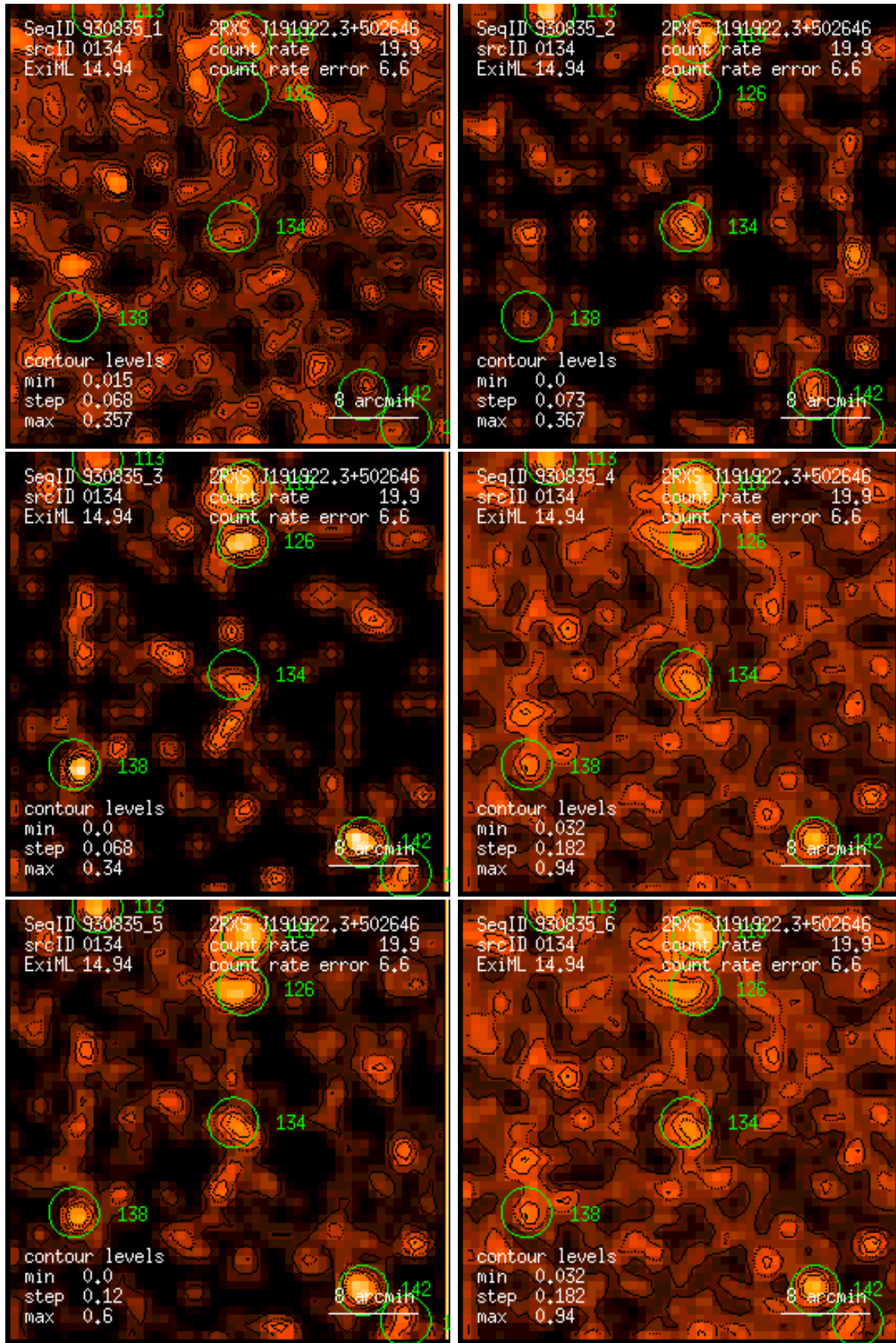
Figure 134: RASS 930835: detection 0134: band rate images, Gaussian filter: (1) PSPC channels 11 – 41, (2) 52 – 90, (3) 91 – 201, (4) 11 – 235, (5) 52 – 201, (6) 11 – 201. Broad band rates in counts/ks. Band rate contour levels in counts/ks/arcmin 2 .
