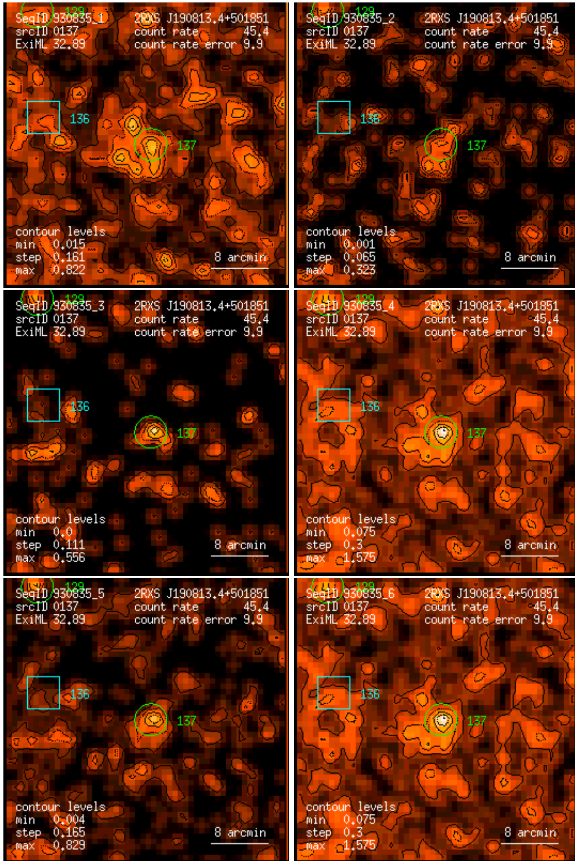
Figure 137: RASS 930835: detection 0137: band rate images, Gaussian filter: (1) PSPC channels 11 – 41, (2) 52 – 90, (3) 91 – 201, (4) 11 – 235, (5) 52 – 201, (6) 11 – 201. Broad band rates in counts/ks. Band rate contour levels in counts/ks/arcmin 2 .
