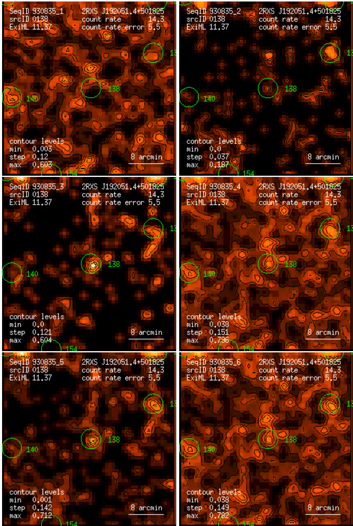
Figure 138: RASS 930835: detection 0138: band rate images, Gaussian filter: (1) PSPC channels 11 – 41, (2) 52 – 90, (3) 91 – 201, (4) 11 – 235, (5) 52 – 201, (6) 11 – 201. Broad band rates in counts/ks. Band rate contour levels in counts/ks/arcmin 2 .
