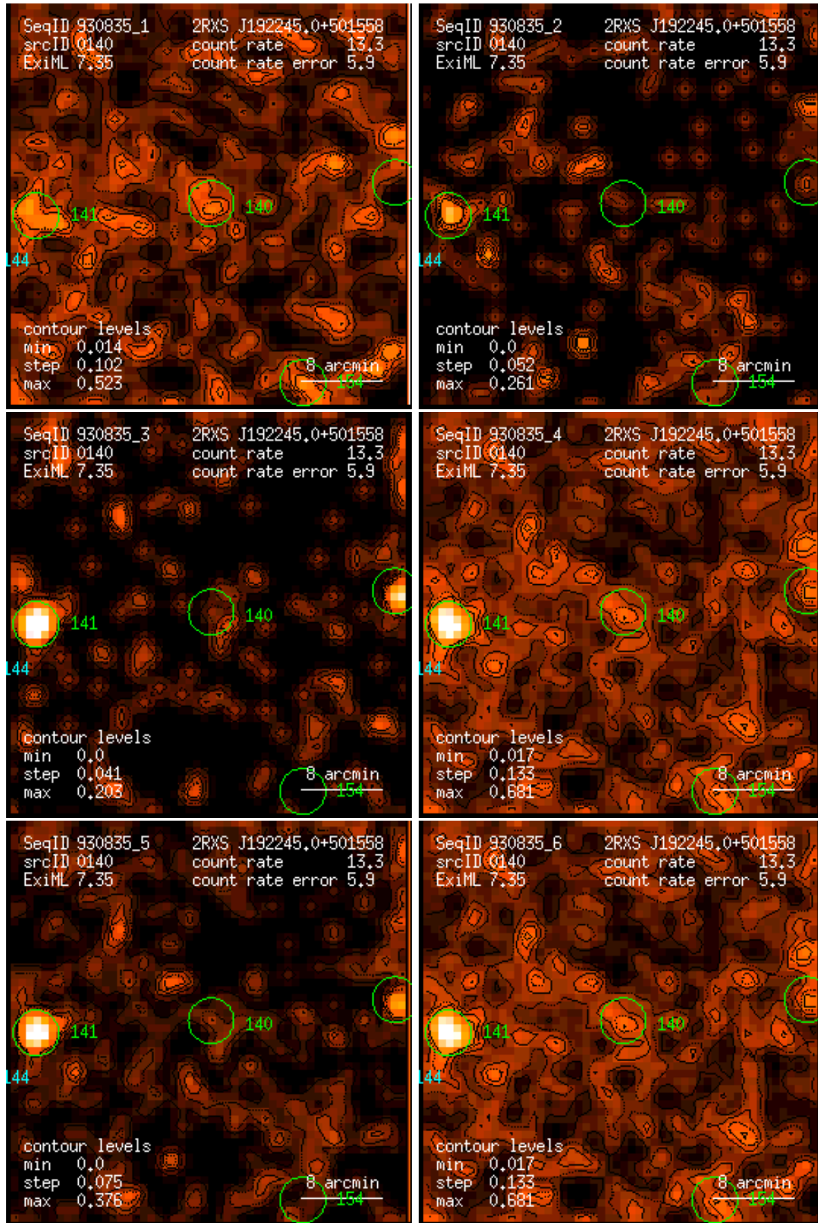
Figure 140: RASS 930835: detection 0140: band rate images, Gaussian filter: (1) PSPC channels 11 – 41, (2) 52 – 90, (3) 91 – 201, (4) 11 – 235, (5) 52 – 201, (6) 11 – 201. Broad band rates in counts/ks. Band rate contour levels in counts/ks/arcmin 2 .
