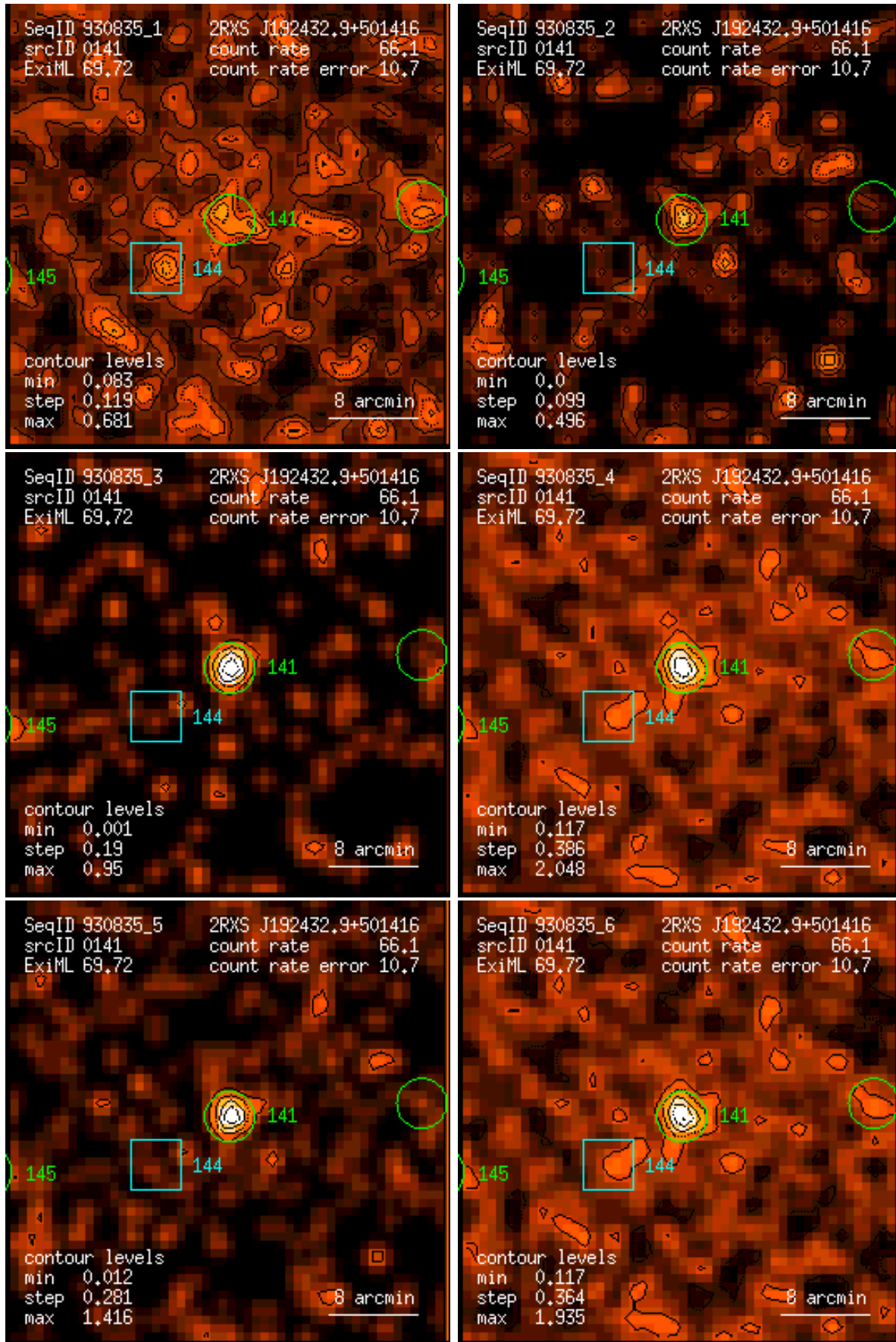
Figure 141: RASS 930835: detection 0141: band rate images, Gaussian filter: (1) PSPC channels 11 – 41, (2) 52 – 90, (3) 91 – 201, (4) 11 – 235, (5) 52 – 201, (6) 11 – 201. Broad band rates in counts/ks. Band rate contour levels in counts/ks/arcmin 2 .
