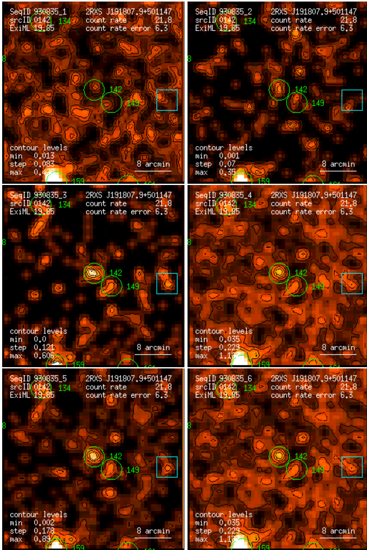
Figure 142: RASS 930835: detection 0142: band rate images, Gaussian filter: (1) PSPC channels 11 – 41, (2) 52 – 90, (3) 91 – 201, (4) 11 – 235, (5) 52 – 201, (6) 11 – 201. Broad band rates in counts/ks. Band rate contour levels in counts/ks/arcmin 2 .
