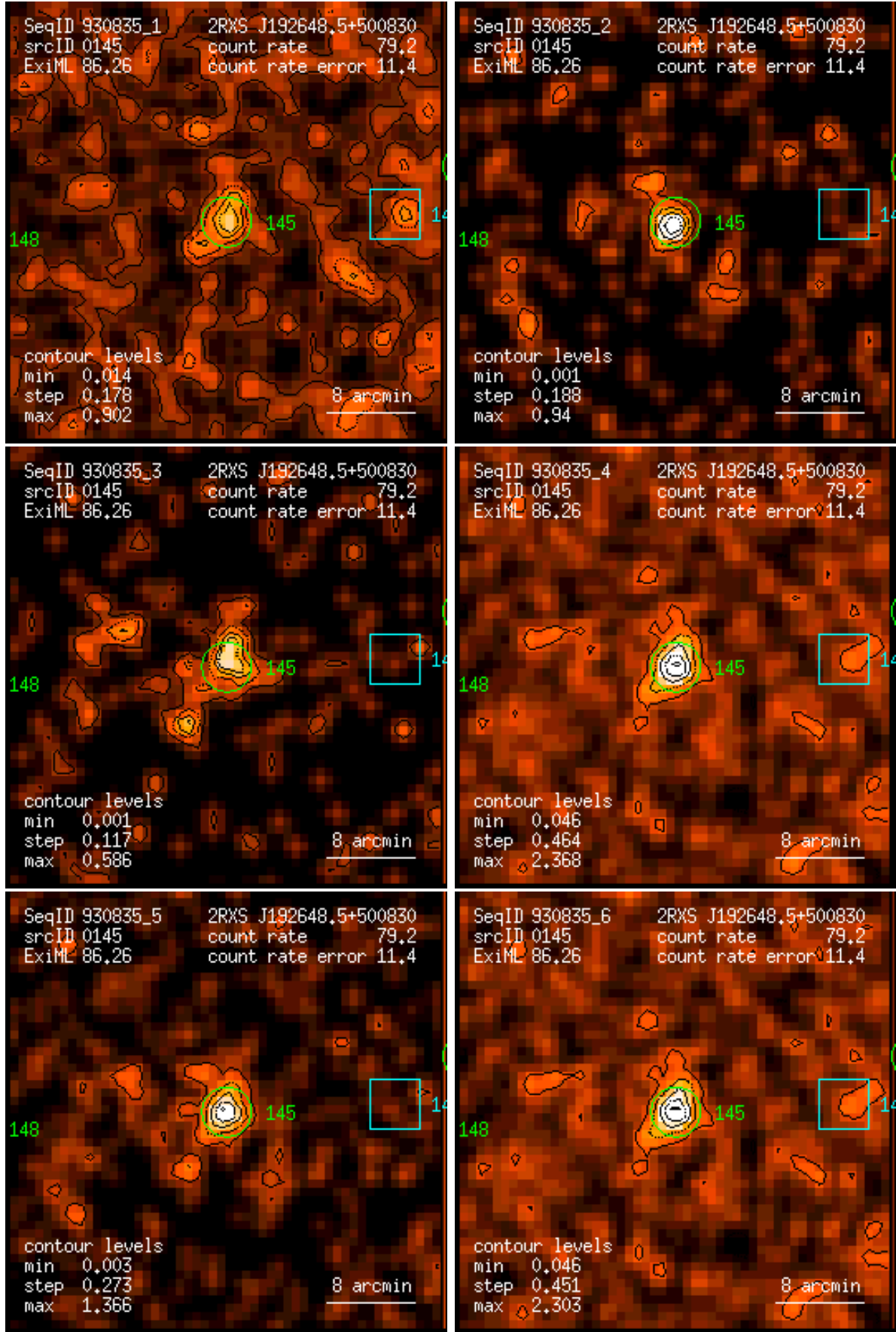
Figure 145: RASS 930835: detection 0145: band rate images, Gaussian filter: (1) PSPC channels 11 – 41, (2) 52 – 90, (3) 91 – 201, (4) 11 – 235, (5) 52 – 201, (6) 11 – 201. Broad band rates in counts/ks. Band rate contour levels in counts/ks/arcmin 2 .
