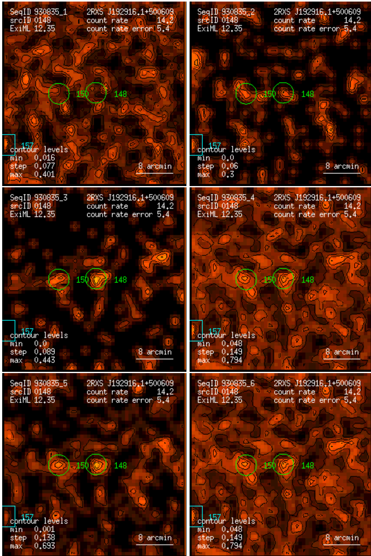
Figure 148: RASS 930835: detection 0148: band rate images, Gaussian filter: (1) PSPC channels 11 – 41, (2) 52 – 90, (3) 91 – 201, (4) 11 – 235, (5) 52 – 201, (6) 11 – 201. Broad band rates in counts/ks. Band rate contour levels in counts/ks/arcmin 2 .
