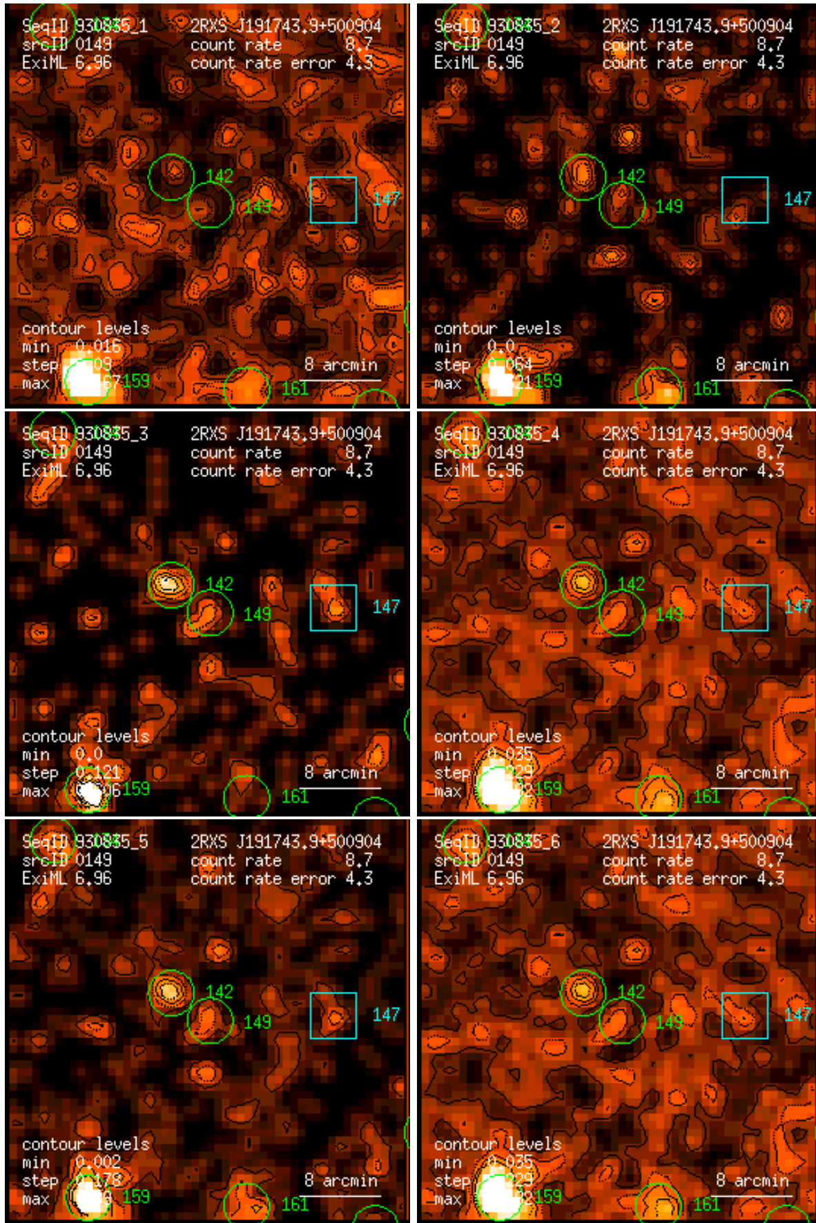
Figure 149: RASS 930835: detection 0149: band rate images, Gaussian filter: (1) PSPC channels 11 – 41, (2) 52 – 90, (3) 91 – 201, (4) 11 – 235, (5) 52 – 201, (6) 11 – 201. Broad band rates in counts/ks. Band rate contour levels in counts/ks/arcmin 2 .
