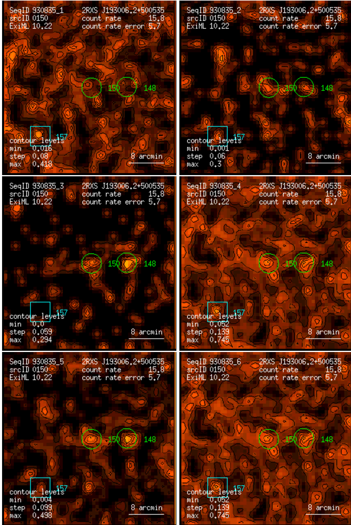
Figure 150: RASS 930835: detection 0150: band rate images, Gaussian filter: (1) PSPC channels 11 – 41, (2) 52 – 90, (3) 91 – 201, (4) 11 – 235, (5) 52 – 201, (6) 11 – 201. Broad band rates in counts/ks. Band rate contour levels in counts/ks/arcmin 2 .
