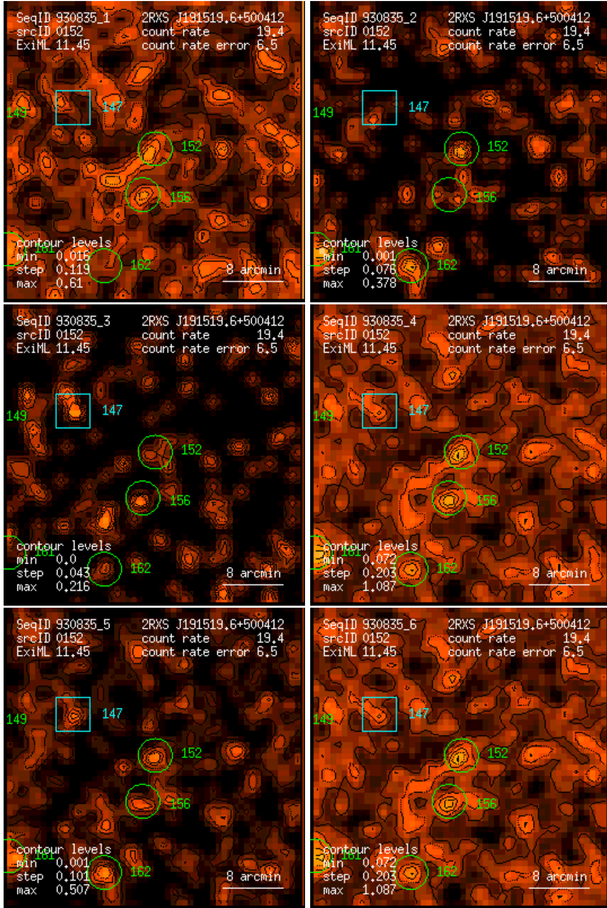
Figure 152: RASS 930835: detection 0152: band rate images, Gaussian filter: (1) PSPC channels 11 – 41, (2) 52 – 90, (3) 91 – 201, (4) 11 – 235, (5) 52 – 201, (6) 11 – 201. Broad band rates in counts/ks. Band rate contour levels in counts/ks/arcmin 2 .
