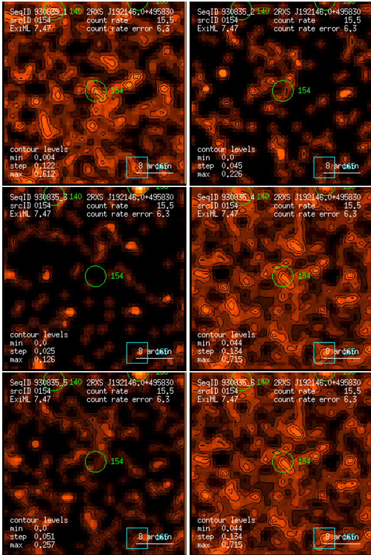
Figure 154: RASS 930835: detection 0154: band rate images, Gaussian filter: (1) PSPC channels 11 – 41, (2) 52 – 90, (3) 91 – 201, (4) 11 – 235, (5) 52 – 201, (6) 11 – 201. Broad band rates in counts/ks. Band rate contour levels in counts/ks/arcmin 2 .
