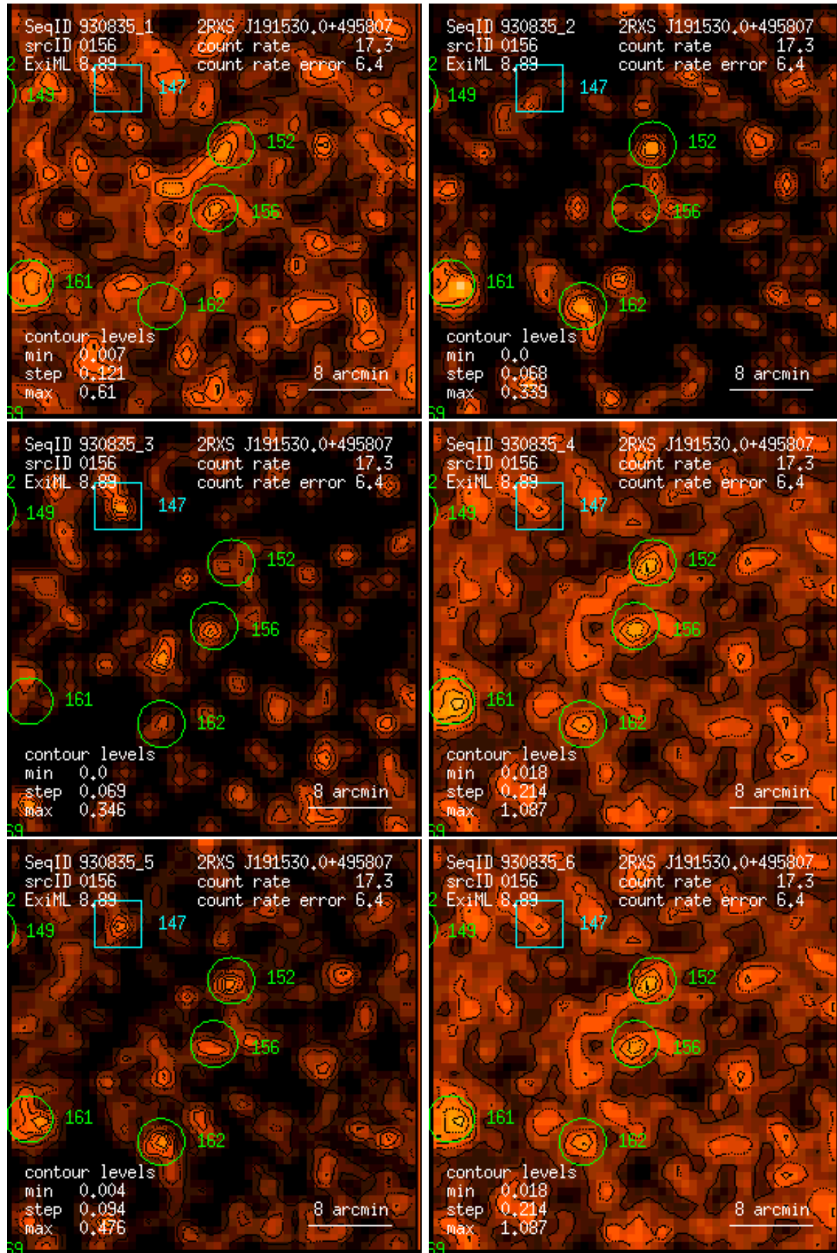
Figure 156: RASS 930835: detection 0156: band rate images, Gaussian filter: (1) PSPC channels 11 – 41, (2) 52 – 90, (3) 91 – 201, (4) 11 – 235, (5) 52 – 201, (6) 11 – 201. Broad band rates in counts/ks. Band rate contour levels in counts/ks/arcmin 2 .
