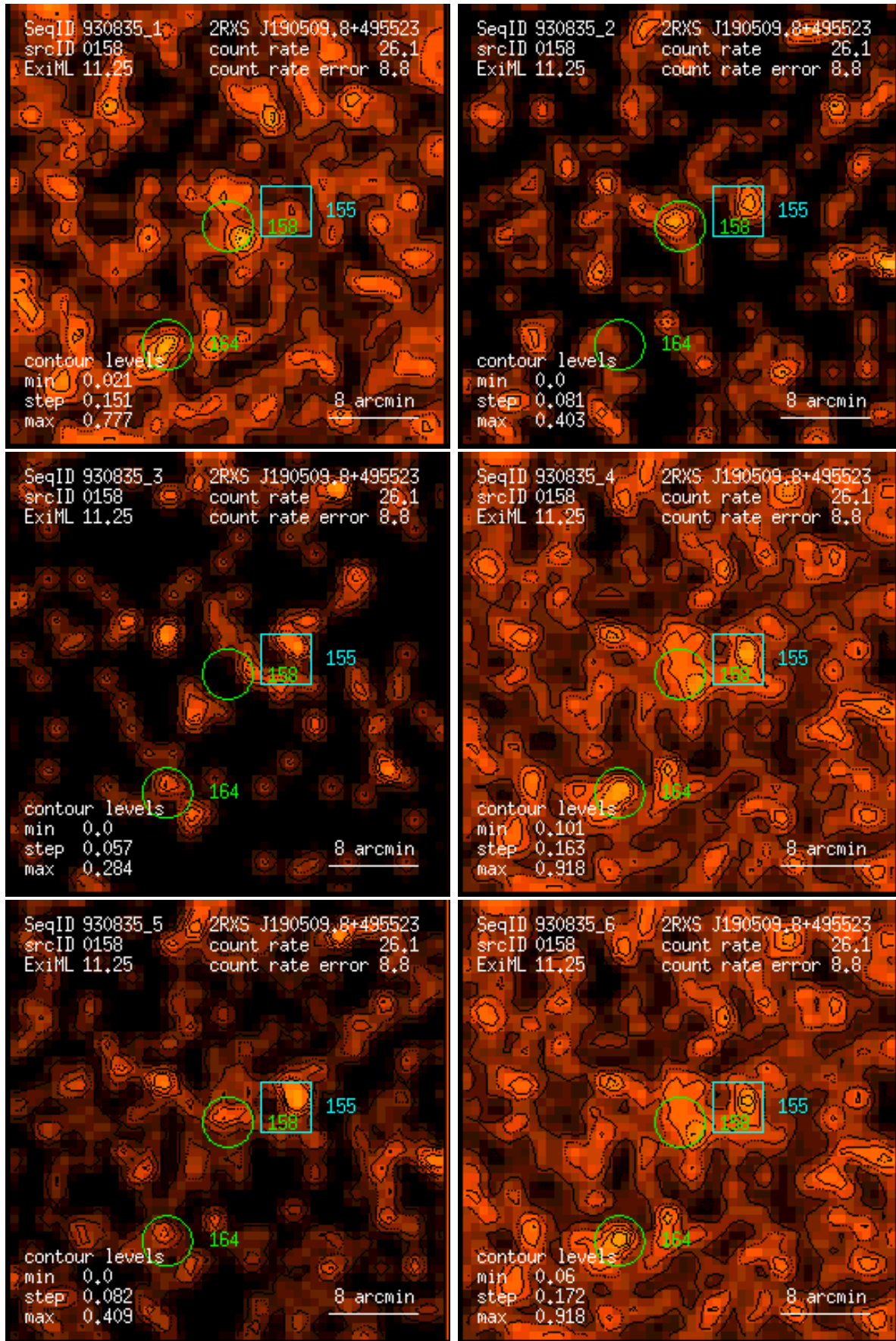
Figure 158: RASS 930835: detection 0158: band rate images, Gaussian filter: (1) PSPC channels 11 – 41, (2) 52 – 90, (3) 91 – 201, (4) 11 – 235, (5) 52 – 201, (6) 11 – 201. Broad band rates in counts/ks. Band rate contour levels in counts/ks/arcmin 2 .
