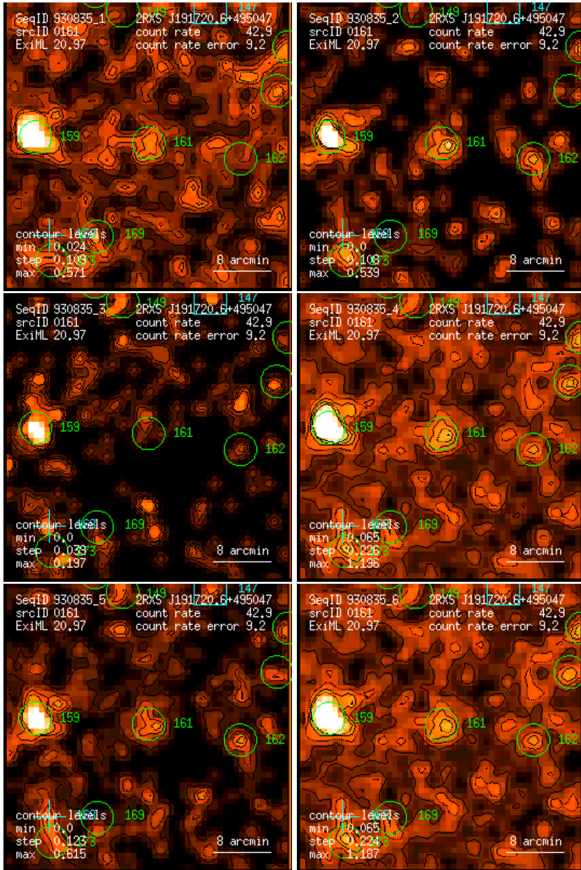
Figure 161: RASS 930835: detection 0161: band rate images, Gaussian filter: (1) PSPC channels 11 – 41, (2) 52 – 90, (3) 91 – 201, (4) 11 – 235, (5) 52 – 201, (6) 11 – 201. Broad band rates in counts/ks. Band rate contour levels in counts/ks/arcmin 2 .
