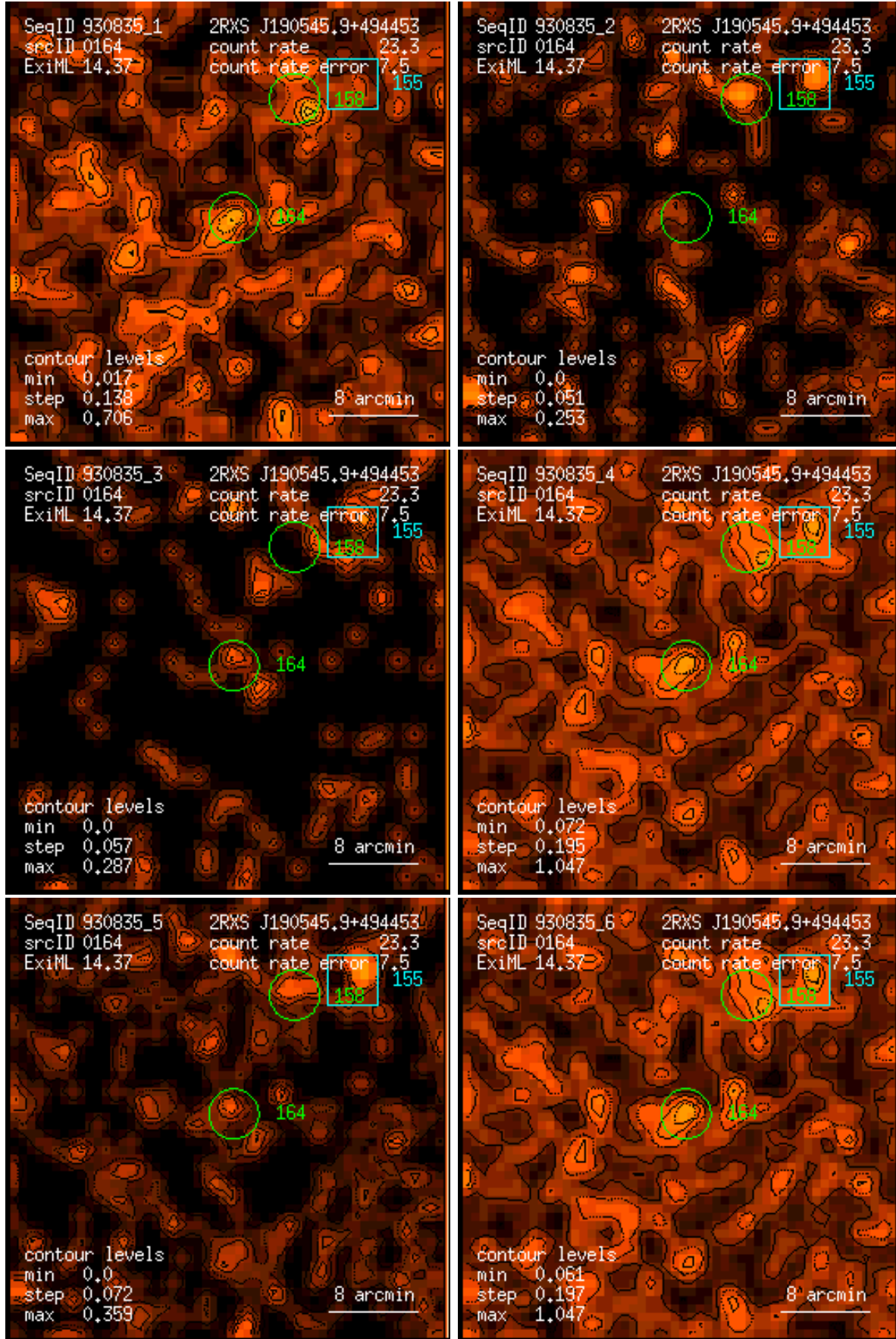
Figure 164: RASS 930835: detection 0164: band rate images, Gaussian filter: (1) PSPC channels 11 – 41, (2) 52 – 90, (3) 91 – 201, (4) 11 – 235, (5) 52 – 201, (6) 11 – 201. Broad band rates in counts/ks. Band rate contour levels in counts/ks/arcmin 2 .
