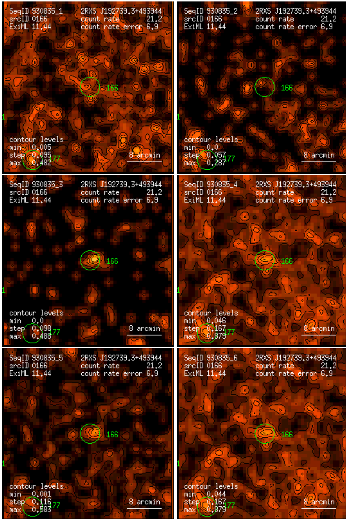
Figure 166: RASS 930835: detection 0166: band rate images, Gaussian filter: (1) PSPC channels 11 – 41, (2) 52 – 90, (3) 91 – 201, (4) 11 – 235, (5) 52 – 201, (6) 11 – 201. Broad band rates in counts/ks. Band rate contour levels in counts/ks/arcmin 2 .
