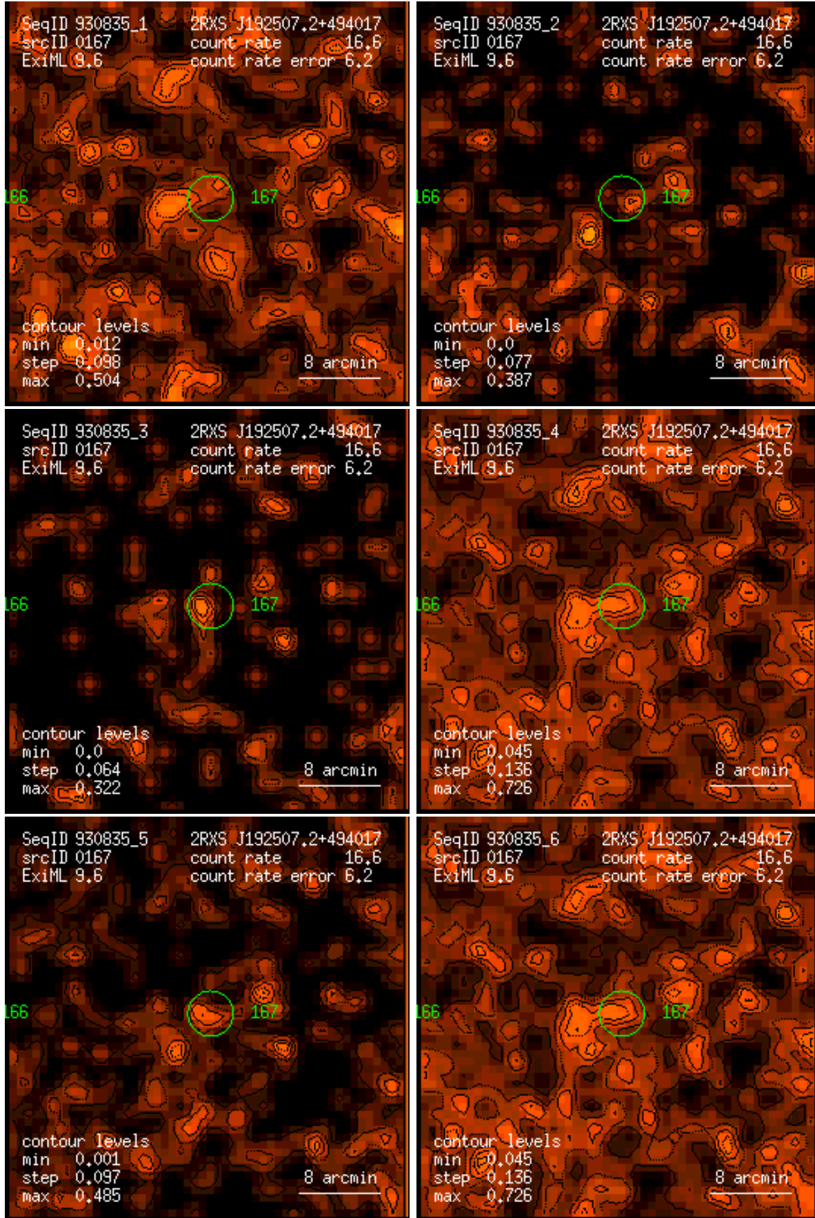
Figure 167: RASS 930835: detection 0167: band rate images, Gaussian filter: (1) PSPC channels 11 – 41, (2) 52 – 90, (3) 91 – 201, (4) 11 – 235, (5) 52 – 201, (6) 11 – 201. Broad band rates in counts/ks. Band rate contour levels in counts/ks/arcmin 2 .
