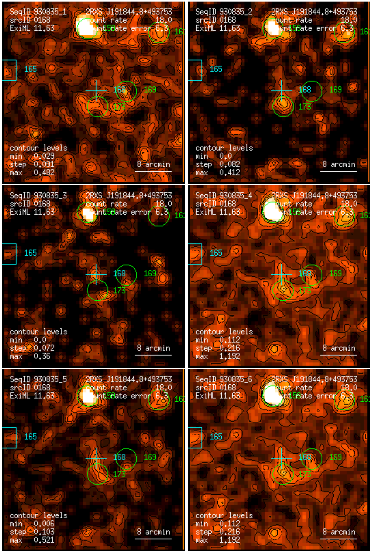
Figure 168: RASS 930835: detection 0168: band rate images, Gaussian filter: (1) PSPC channels 11 – 41, (2) 52 – 90, (3) 91 – 201, (4) 11 – 235, (5) 52 – 201, (6) 11 – 201. Broad band rates in counts/ks. Band rate contour levels in counts/ks/arcmin 2 .
