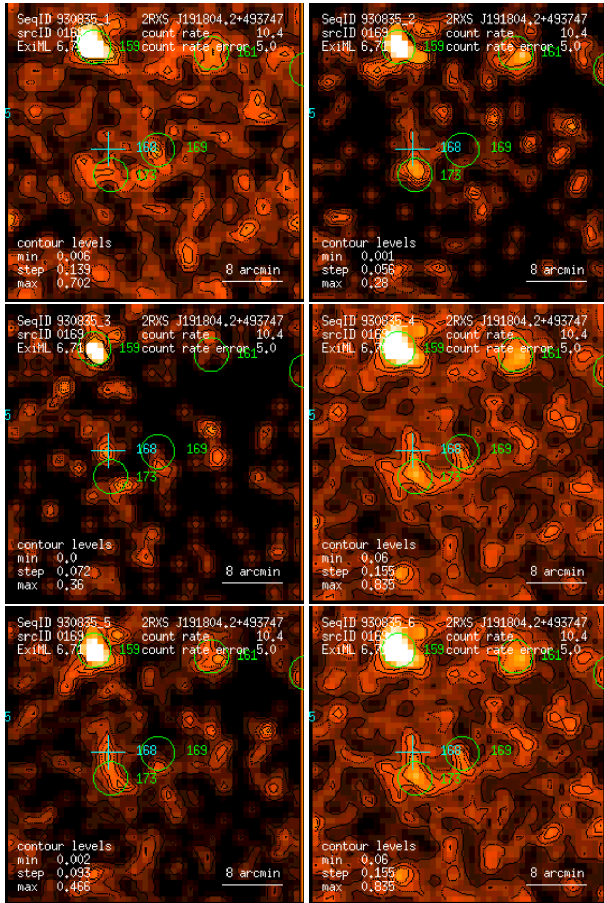
Figure 169: RASS 930835: detection 0169: band rate images, Gaussian filter: (1) PSPC channels 11 – 41, (2) 52 – 90, (3) 91 – 201, (4) 11 – 235, (5) 52 – 201, (6) 11 – 201. Broad band rates in counts/ks. Band rate contour levels in counts/ks/arcmin 2 .
