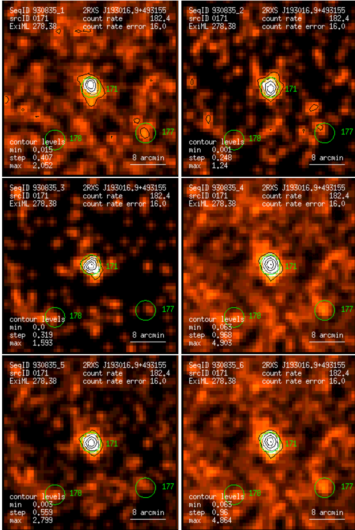
Figure 171: RASS 930835: detection 0171: band rate images, Gaussian filter: (1) PSPC channels 11 – 41, (2) 52 – 90, (3) 91 – 201, (4) 11 – 235, (5) 52 – 201, (6) 11 – 201. Broad band rates in counts/ks. Band rate contour levels in counts/ks/arcmin 2 .
