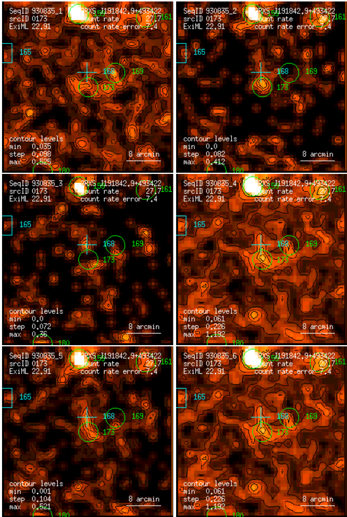
Figure 173: RASS 930835: detection 0173: band rate images, Gaussian filter: (1) PSPC channels 11 – 41, (2) 52 – 90, (3) 91 – 201, (4) 11 – 235, (5) 52 – 201, (6) 11 – 201. Broad band rates in counts/ks. Band rate contour levels in counts/ks/arcmin 2 .
