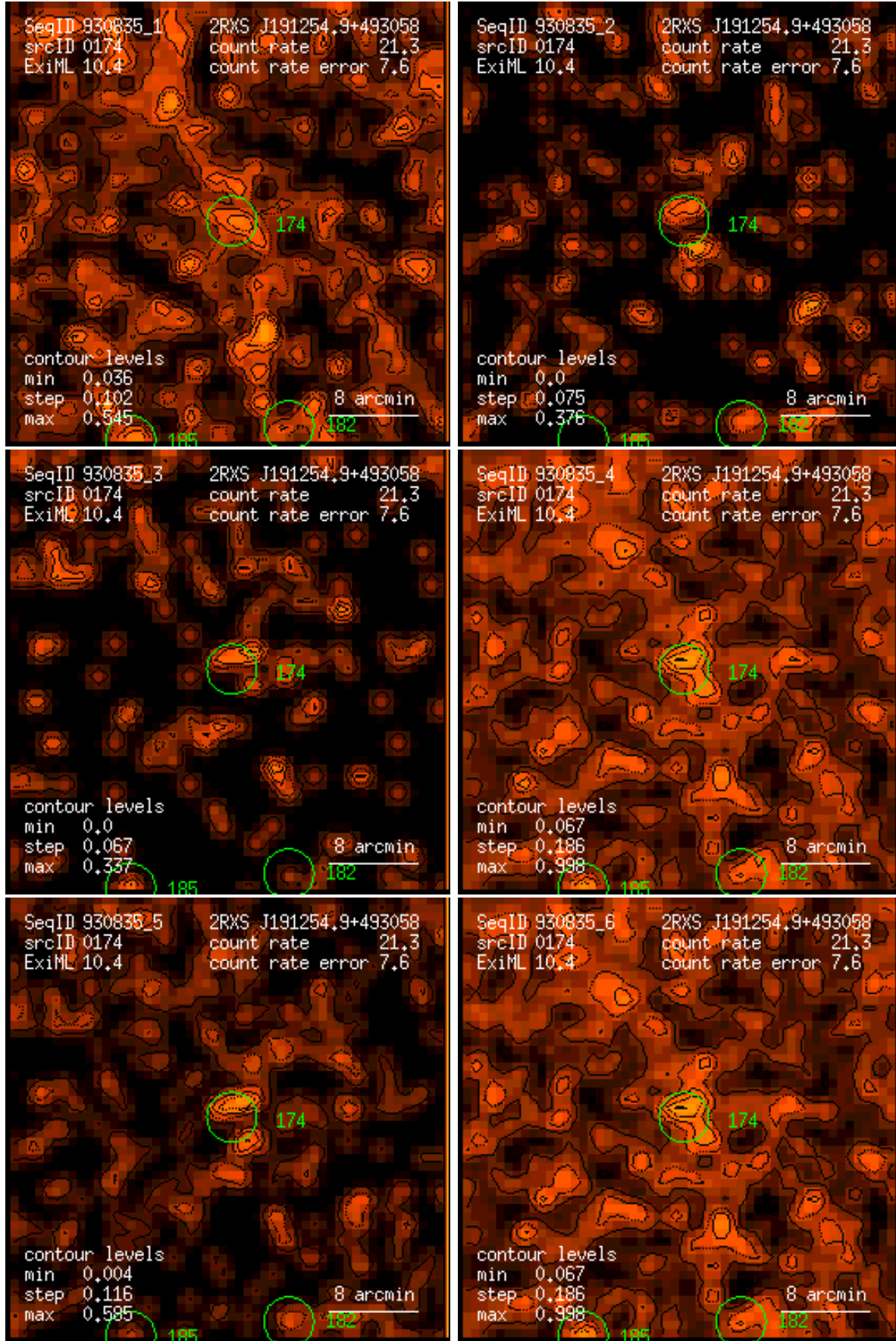
Figure 174: RASS 930835: detection 0174: band rate images, Gaussian filter: (1) PSPC channels 11 – 41, (2) 52 – 90, (3) 91 – 201, (4) 11 – 235, (5) 52 – 201, (6) 11 – 201. Broad band rates in counts/ks. Band rate contour levels in counts/ks/arcmin 2 .
