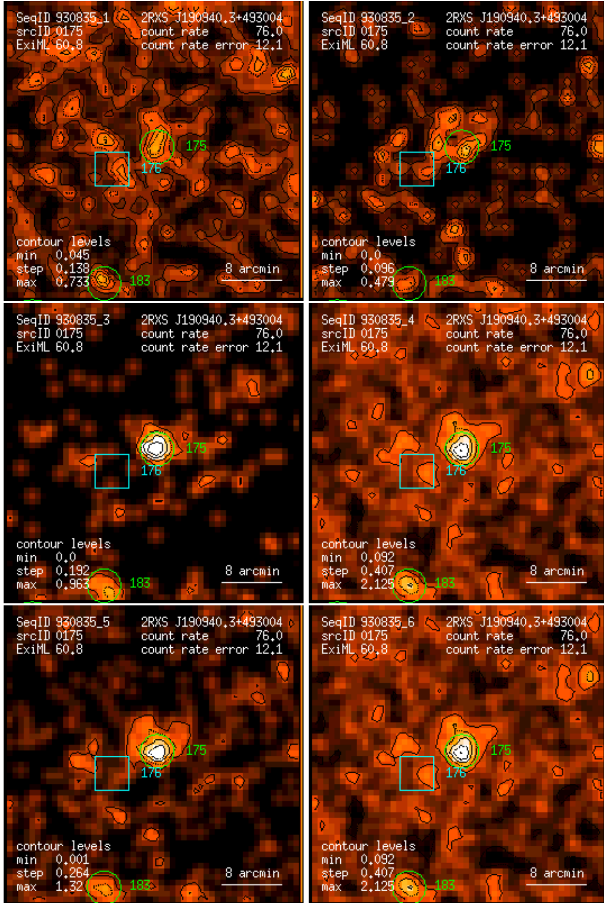
Figure 175: RASS 930835: detection 0175: band rate images, Gaussian filter: (1) PSPC channels 11 – 41, (2) 52 – 90, (3) 91 – 201, (4) 11 – 235, (5) 52 – 201, (6) 11 – 201. Broad band rates in counts/ks. Band rate contour levels in counts/ks/arcmin 2 .
