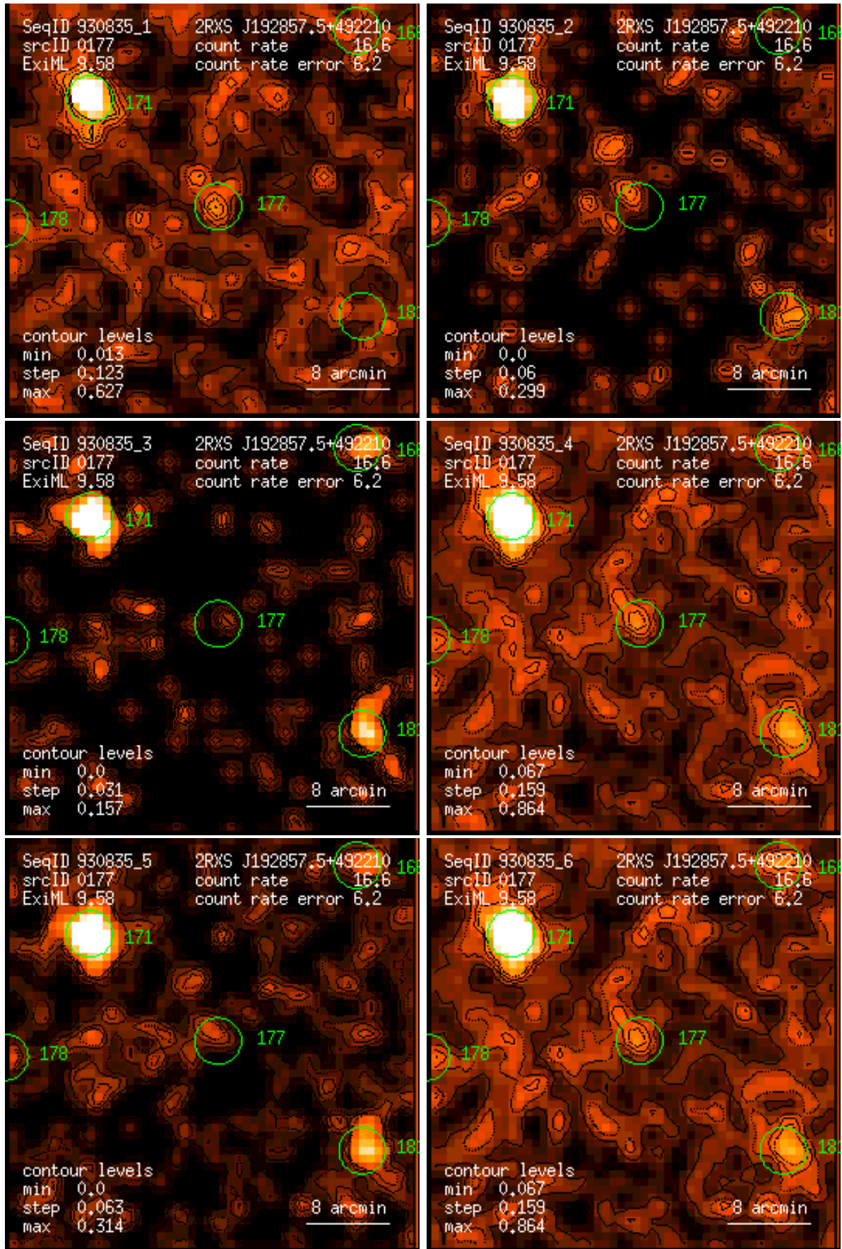
Figure 177: RASS 930835: detection 0177: band rate images, Gaussian filter: (1) PSPC channels 11 – 41, (2) 52 – 90, (3) 91 – 201, (4) 11 – 235, (5) 52 – 201, (6) 11 – 201. Broad band rates in counts/ks. Band rate contour levels in counts/ks/arcmin 2 .
