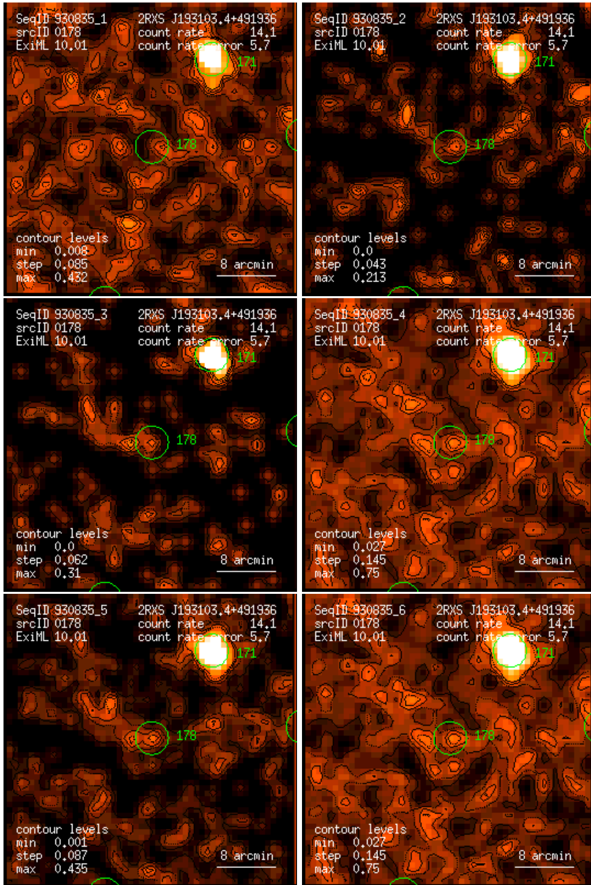
Figure 178: RASS 930835: detection 0178: band rate images, Gaussian filter: (1) PSPC channels 11 – 41, (2) 52 – 90, (3) 91 – 201, (4) 11 – 235, (5) 52 – 201, (6) 11 – 201. Broad band rates in counts/ks. Band rate contour levels in counts/ks/arcmin 2 .
