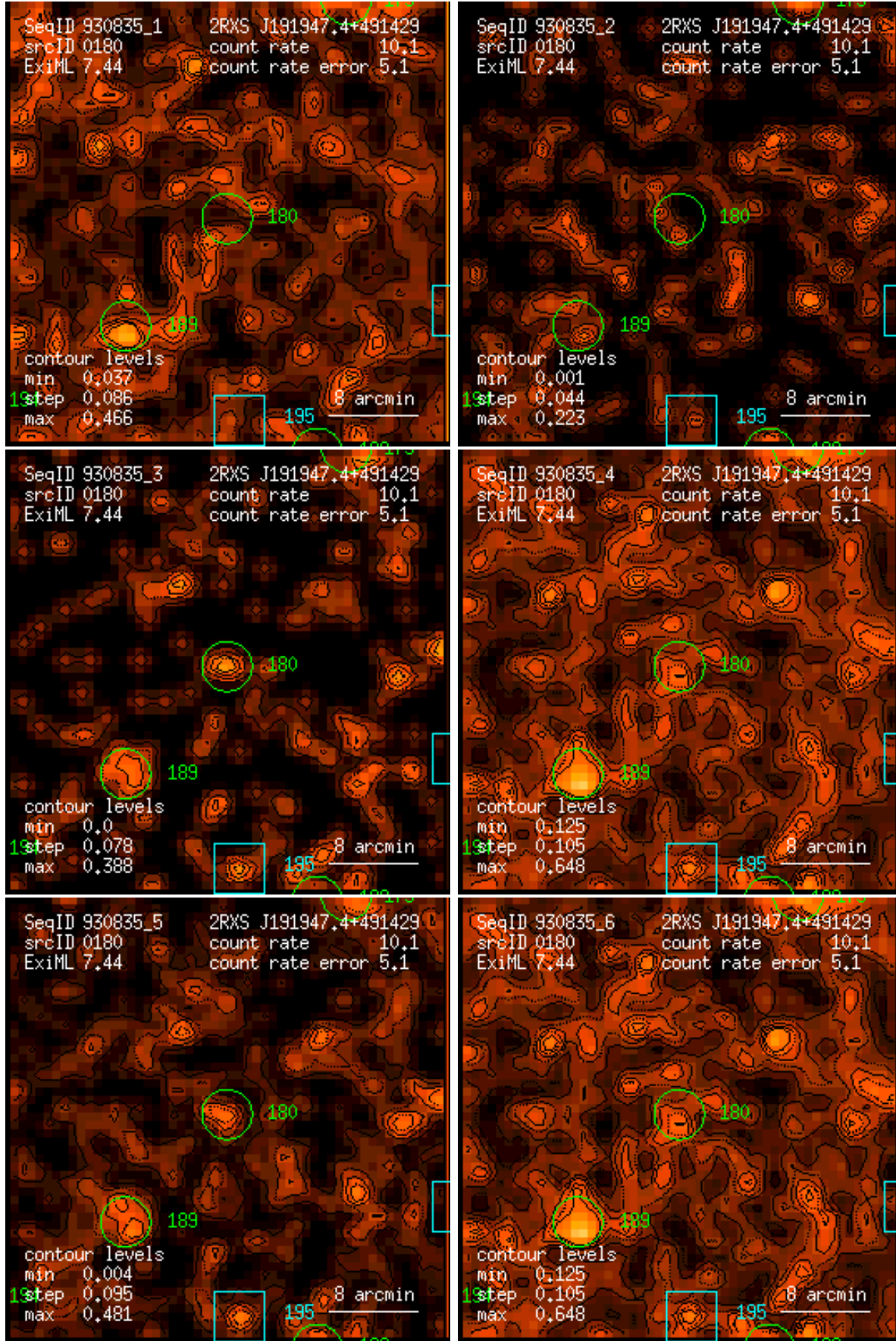
Figure 180: RASS 930835: detection 0180: band rate images, Gaussian filter: (1) PSPC channels 11 – 41, (2) 52 – 90, (3) 91 – 201, (4) 11 – 235, (5) 52 – 201, (6) 11 – 201. Broad band rates in counts/ks. Band rate contour levels in counts/ks/arcmin 2 .
