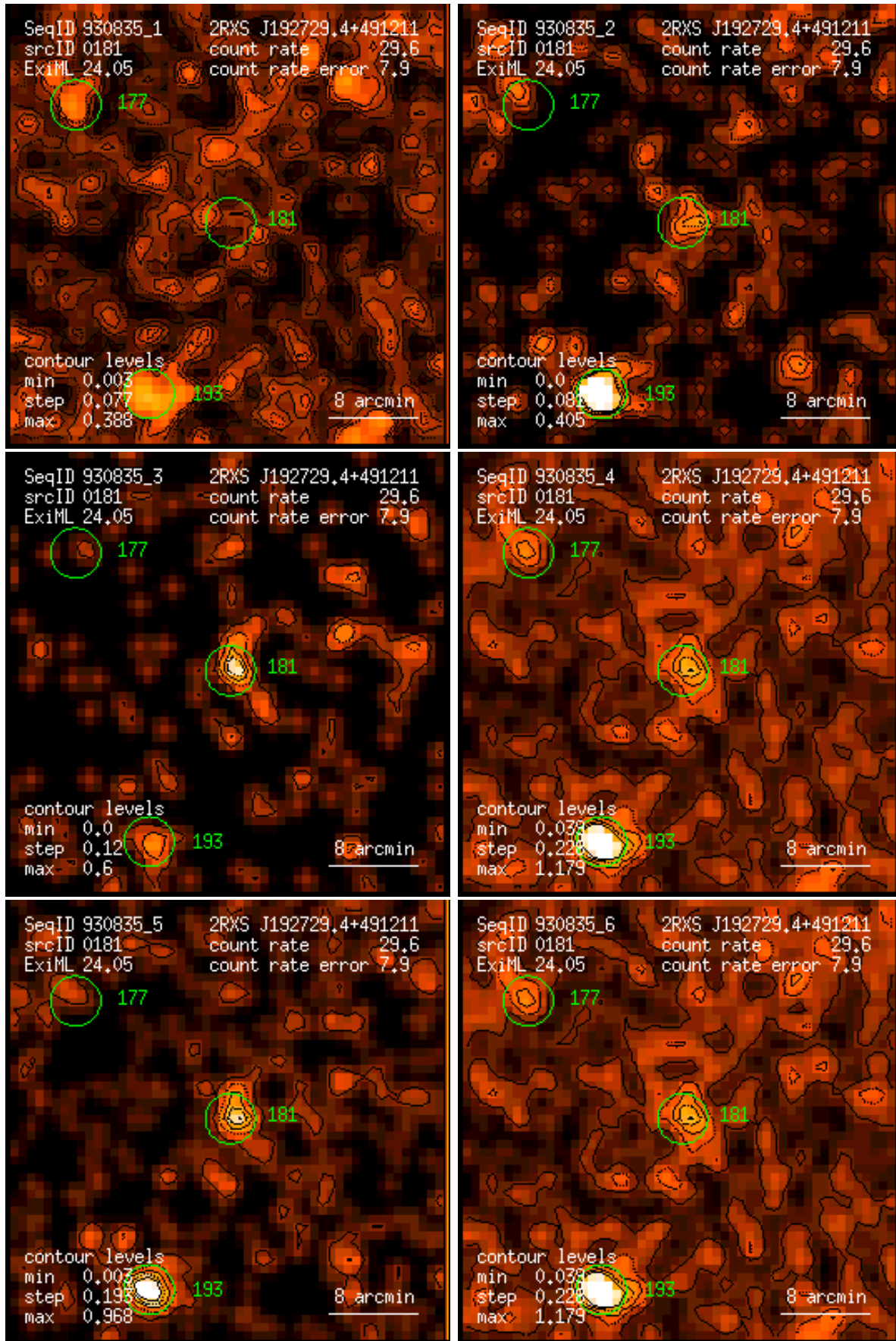
Figure 181: RASS 930835: detection 0181: band rate images, Gaussian filter: (1) PSPC channels 11 – 41, (2) 52 – 90, (3) 91 – 201, (4) 11 – 235, (5) 52 – 201, (6) 11 – 201. Broad band rates in counts/ks. Band rate contour levels in counts/ks/arcmin 2 .
