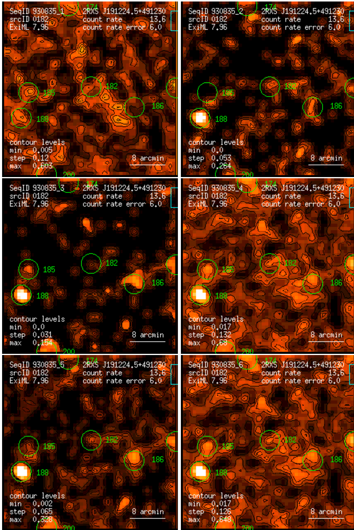
Figure 182: RASS 930835: detection 0182: band rate images, Gaussian filter: (1) PSPC channels 11 – 41, (2) 52 – 90, (3) 91 – 201, (4) 11 – 235, (5) 52 – 201, (6) 11 – 201. Broad band rates in counts/ks. Band rate contour levels in counts/ks/arcmin 2 .
