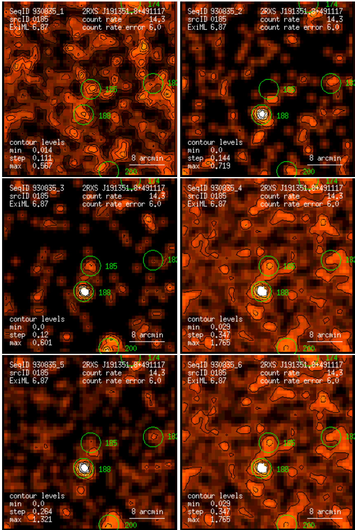
Figure 185: RASS 930835: detection 0185: band rate images, Gaussian filter: (1) PSPC channels 11 – 41, (2) 52 – 90, (3) 91 – 201, (4) 11 – 235, (5) 52 – 201, (6) 11 – 201. Broad band rates in counts/ks. Band rate contour levels in counts/ks/arcmin 2 .
