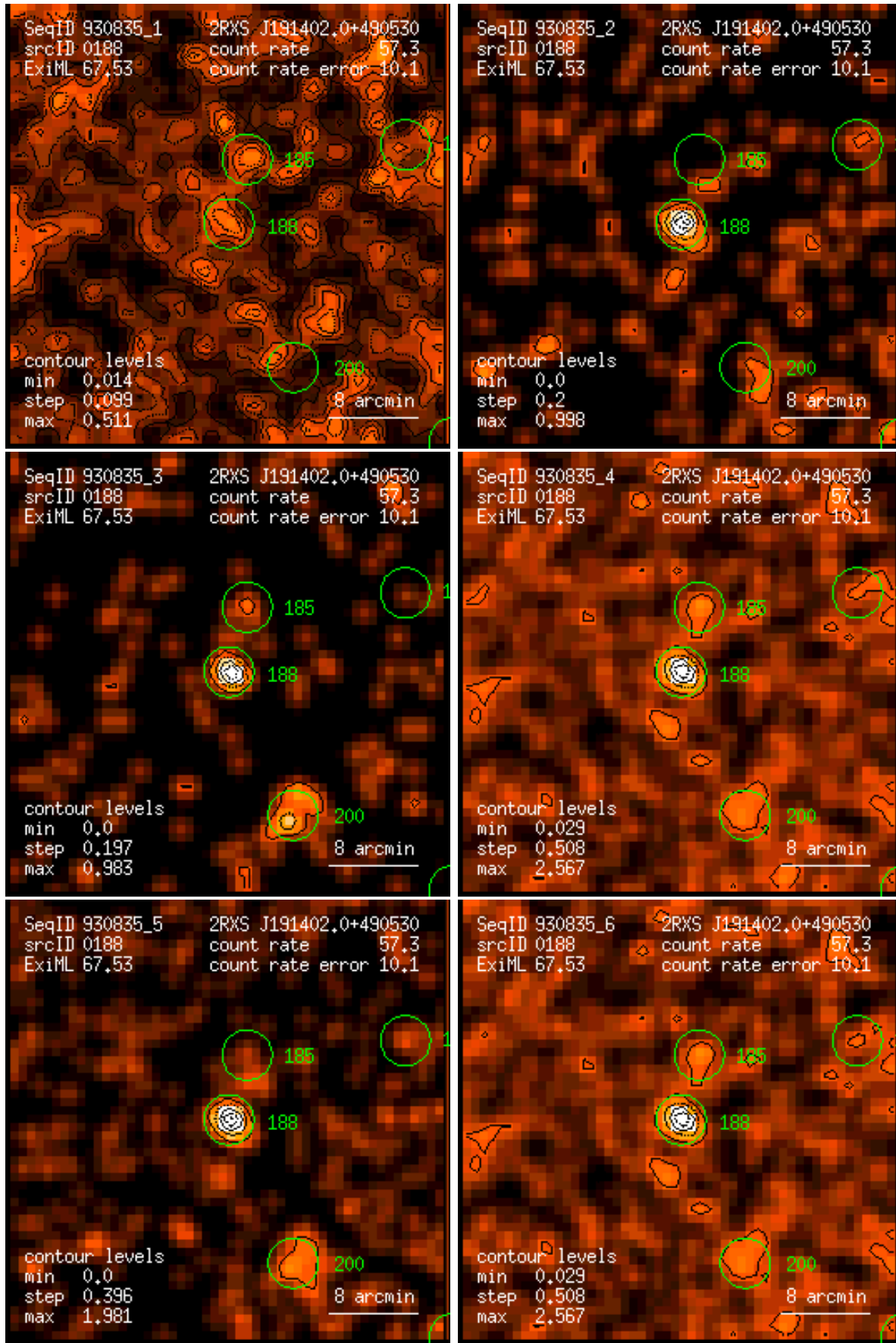
Figure 188: RASS 930835: detection 0188: band rate images, Gaussian filter: (1) PSPC channels 11 – 41, (2) 52 – 90, (3) 91 – 201, (4) 11 – 235, (5) 52 – 201, (6) 11 – 201. Broad band rates in counts/ks. Band rate contour levels in counts/ks/arcmin 2 .
