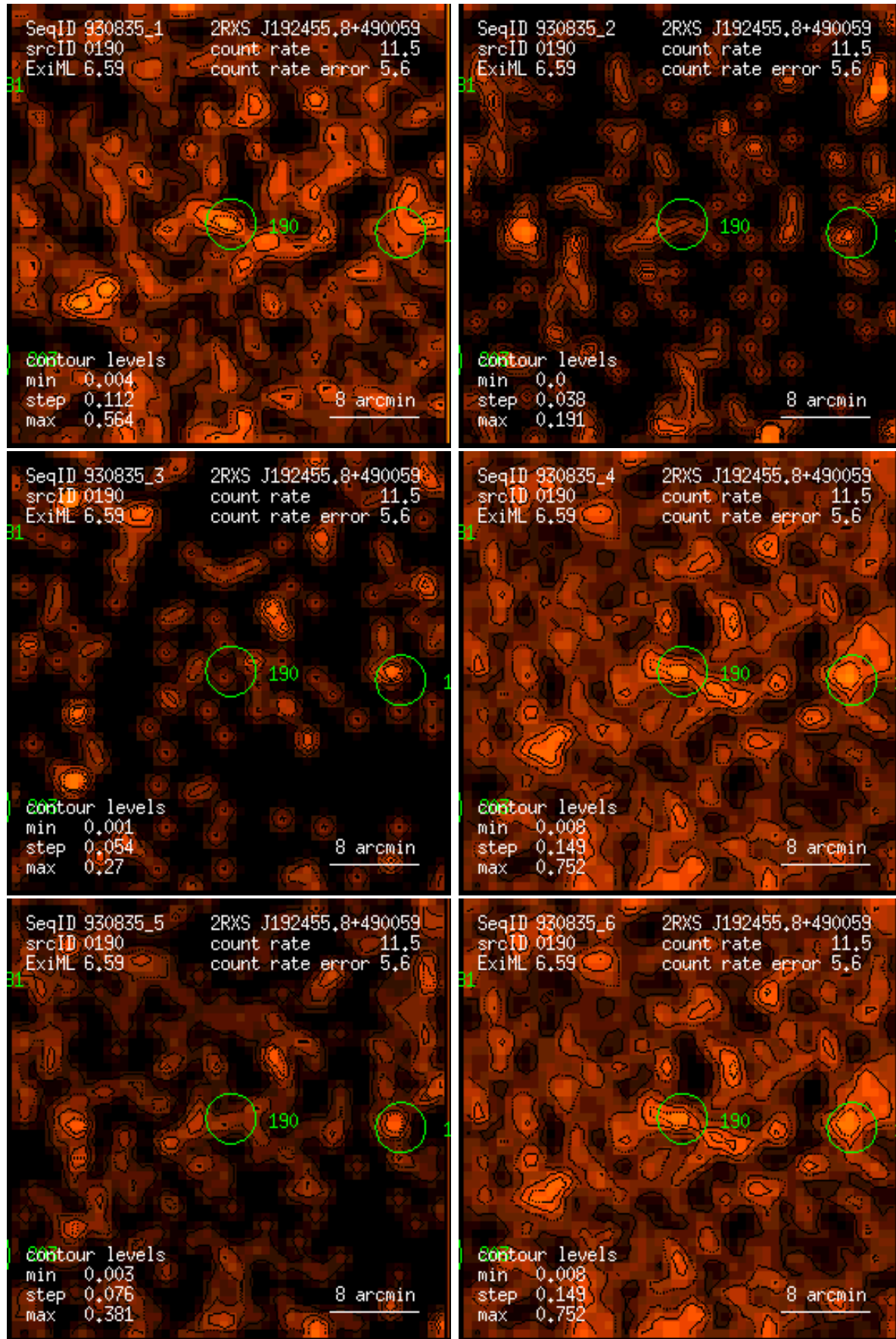
Figure 190: RASS 930835: detection 0190: band rate images, Gaussian filter: (1) PSPC channels 11 – 41, (2) 52 – 90, (3) 91 – 201, (4) 11 – 235, (5) 52 – 201, (6) 11 – 201. Broad band rates in counts/ks. Band rate contour levels in counts/ks/arcmin 2 .
